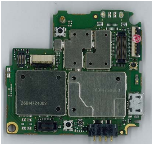
Main Board Bottom With Shields
