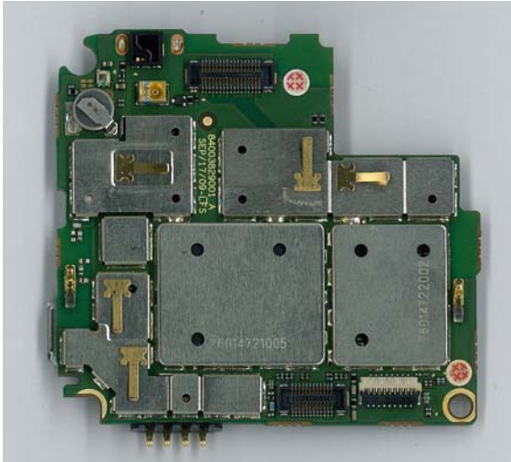
Main Board Top With shields
