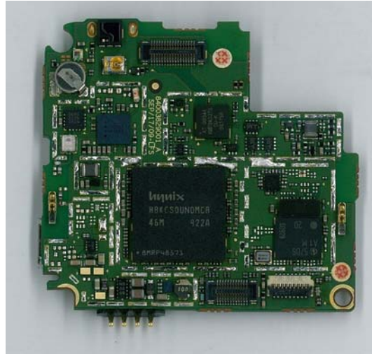
Main Board Top Without shields
