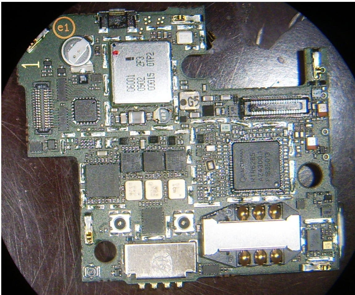
Main Board Bottom Side without Shields
