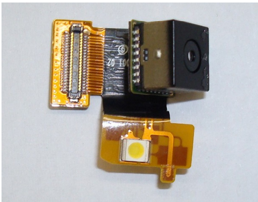
Imager and Flex
