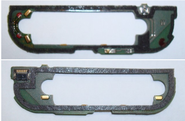
Antenna PCB Bottom and Top
