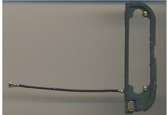
Antenna PCB With Coax
