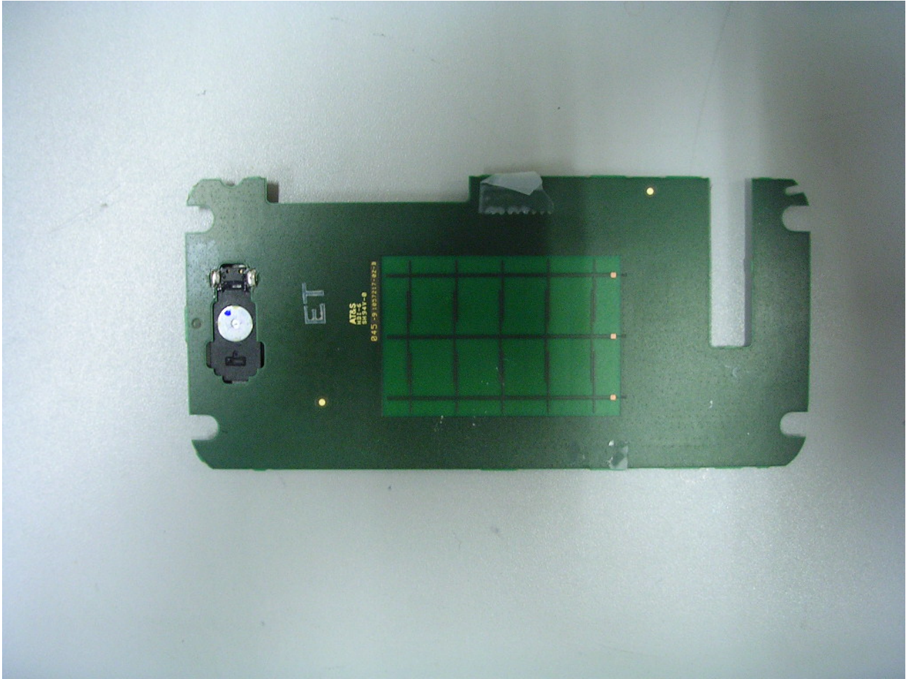
Flip Board Bottom Side with No Shields
