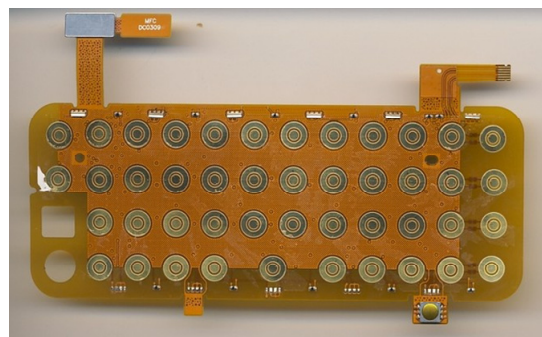
Keyboard Flex (no popples)
