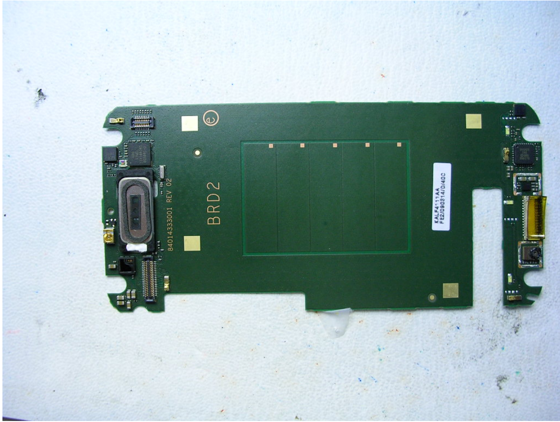
Flip Board Top Side with No Shields
