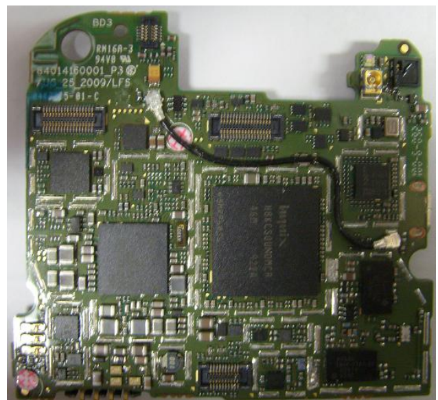
Main Board Bottom W/O shields
