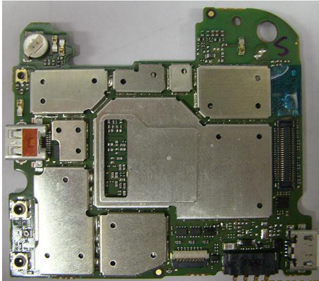
Main Board Top W/ Shields
