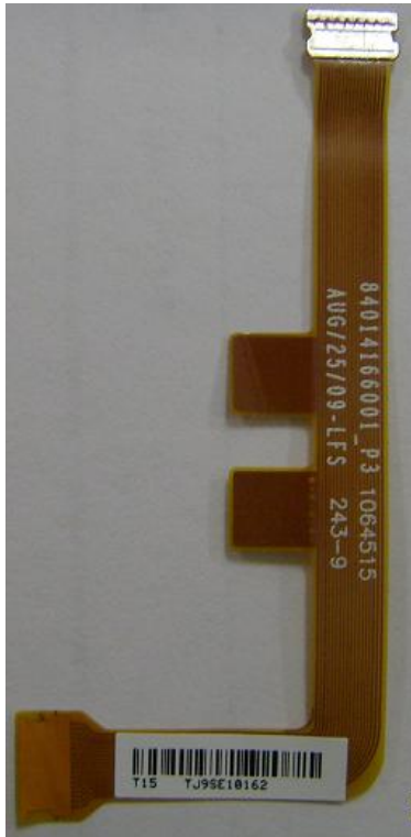
LCD Bridge Flex Top
