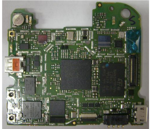
Main Board Top W/O Shields
