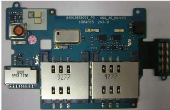
Daughter Board Top W/ shields
