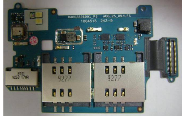
Daughter Board Top W/O shields
