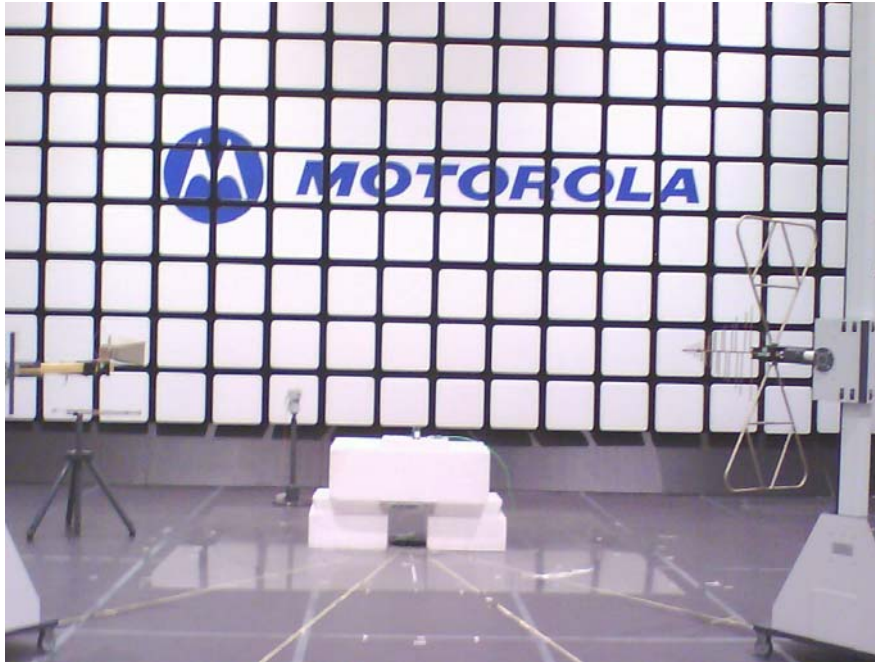
Radiated Emissions
