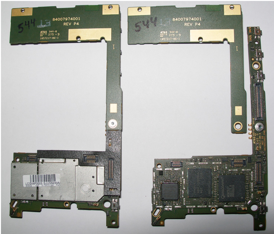
PCB Side 1 With Shields
