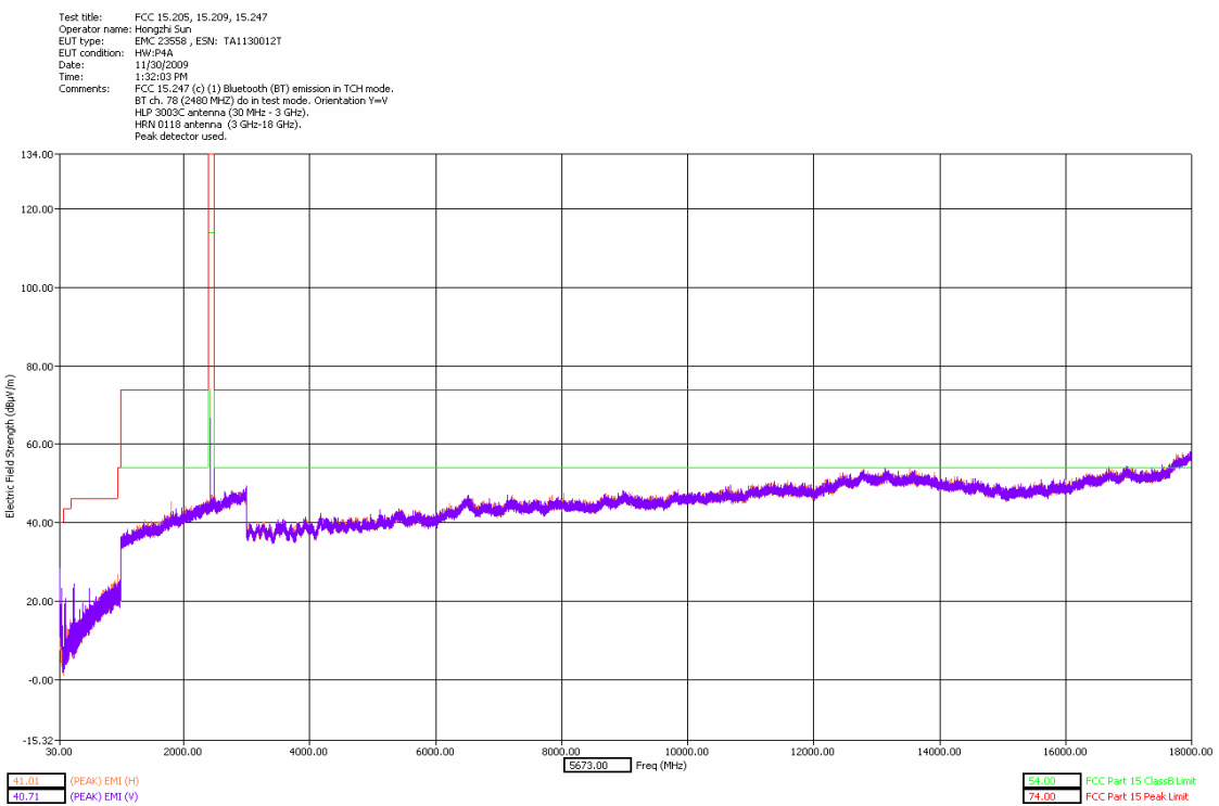
30 MHz – 18 GHz High Channel Dual Polarization Y
