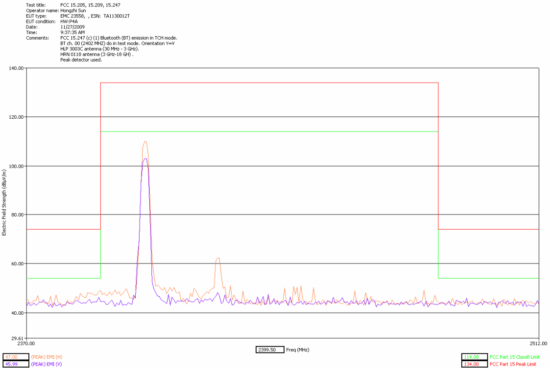
Authorized Band Emissions Low Channel Dual Polarization Y
