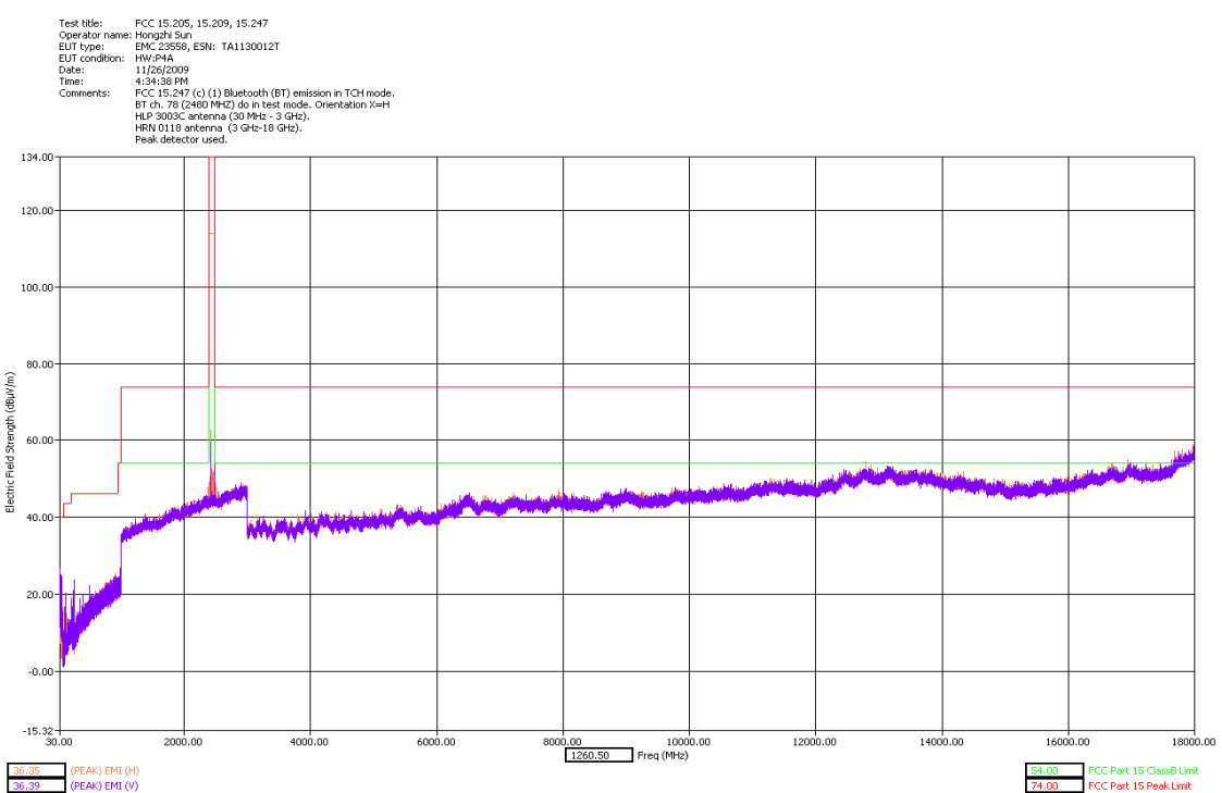
30 MHz – 18 GHz High Channel Dual Polarization X
