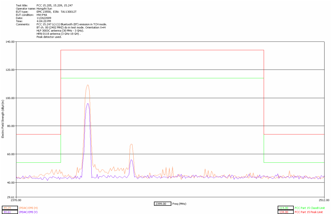
Authorized Band Emissions Low Channel Dual Polarization X
