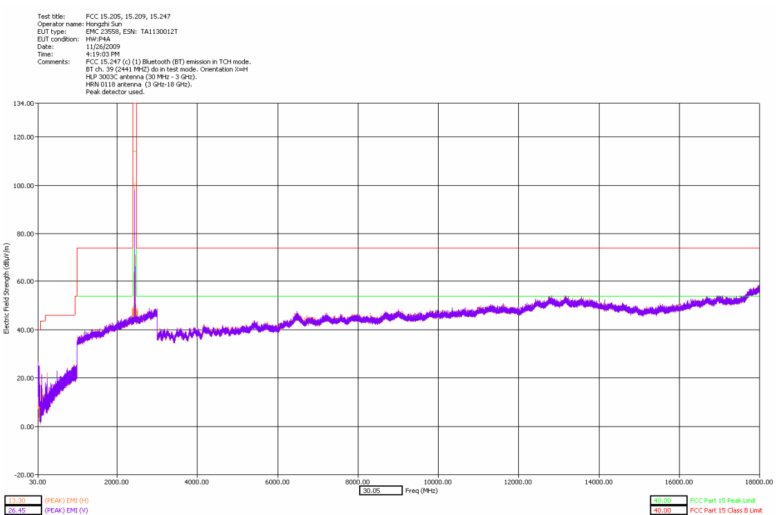
30 MHz – 18 GHz Middle Channel Dual Polarization X
