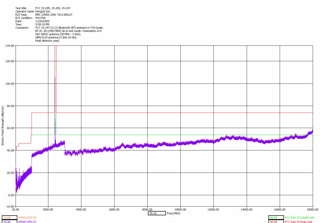
30 MHz – 18 GHz Low Channel Dual Polarization Z
