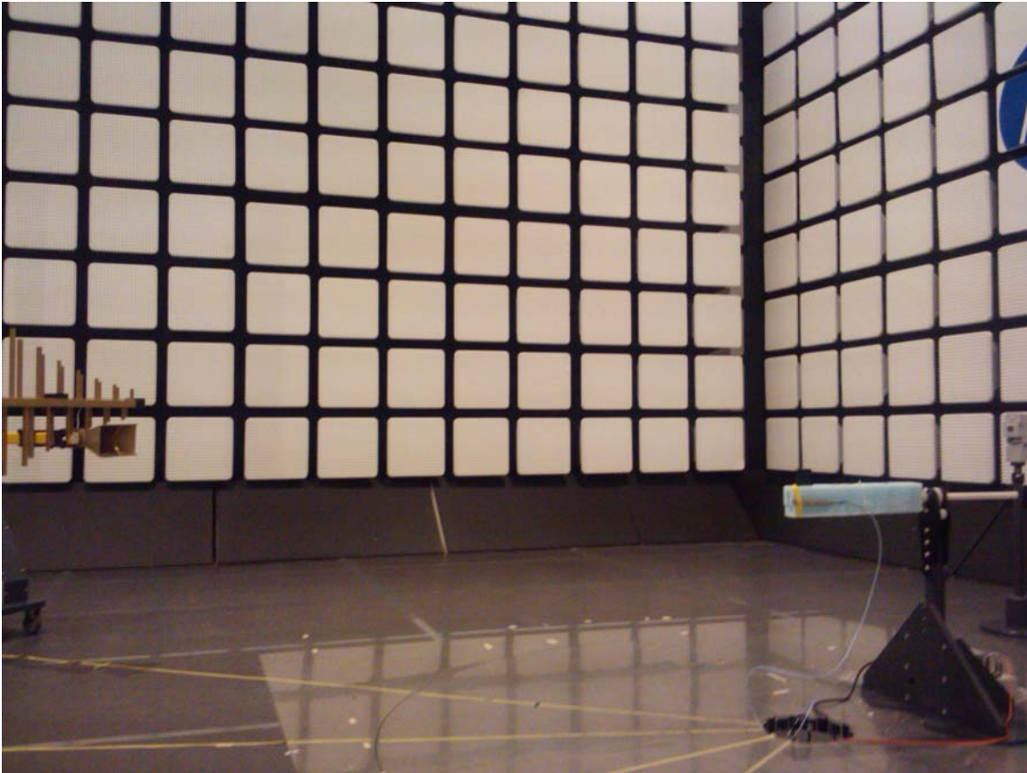
Radiated Emissions – BT & WLAN - BJ
