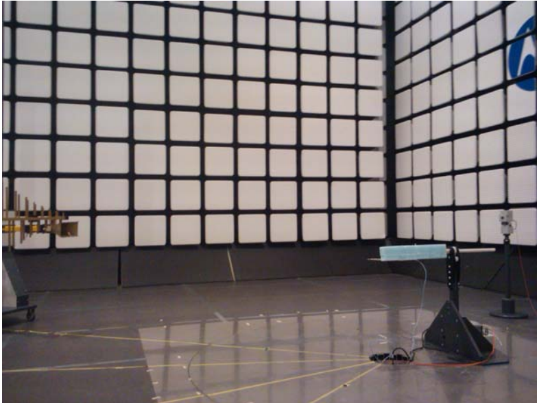
TX Radiated Emissions – GSM, BT & WLAN
