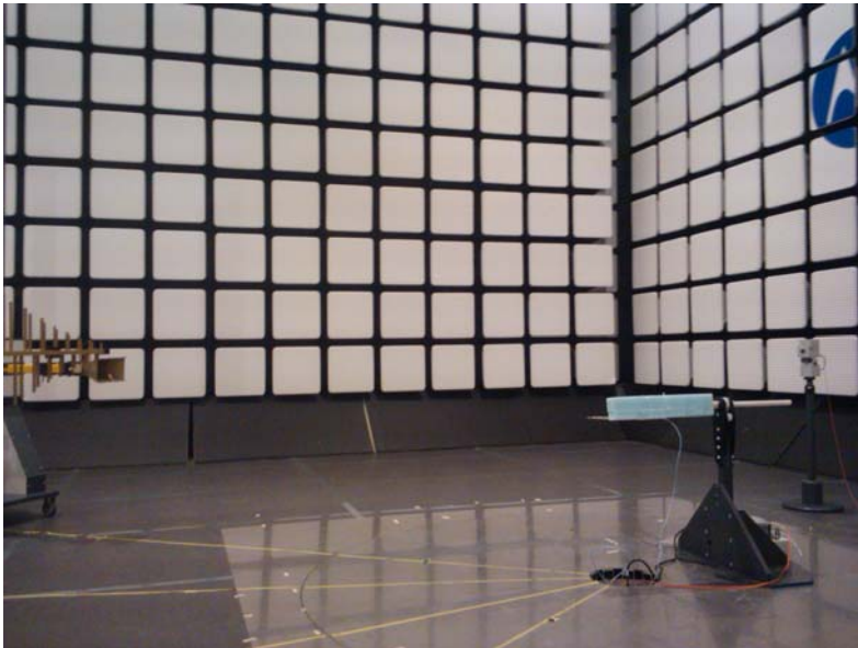
TX Radiated Emissions
