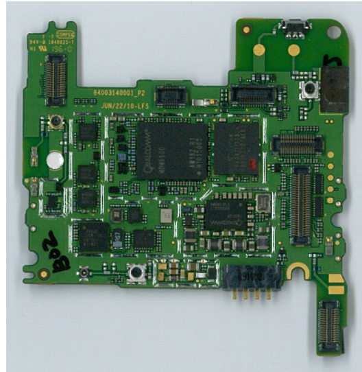
Main Board Top Without shields
