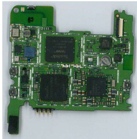
Main Board Bottom Without Shields
