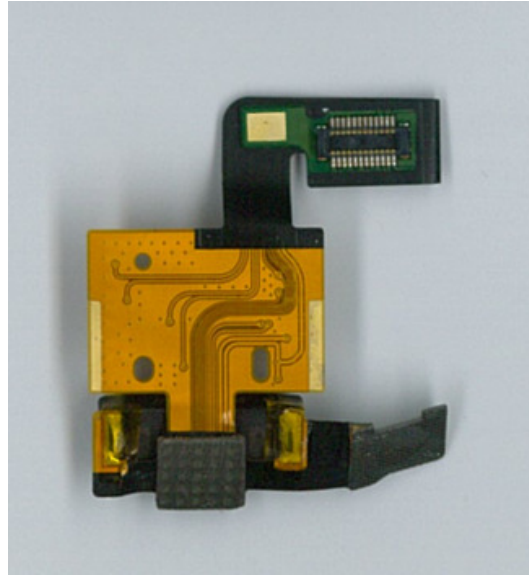
Headset Jack Flex Bottom
