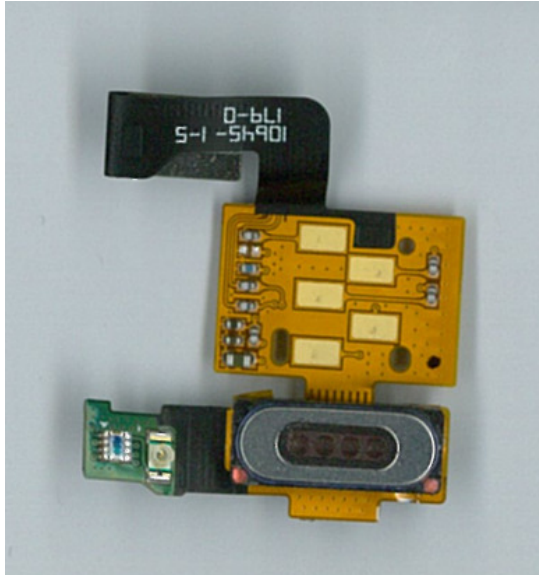
Headset Jack Flex Top
