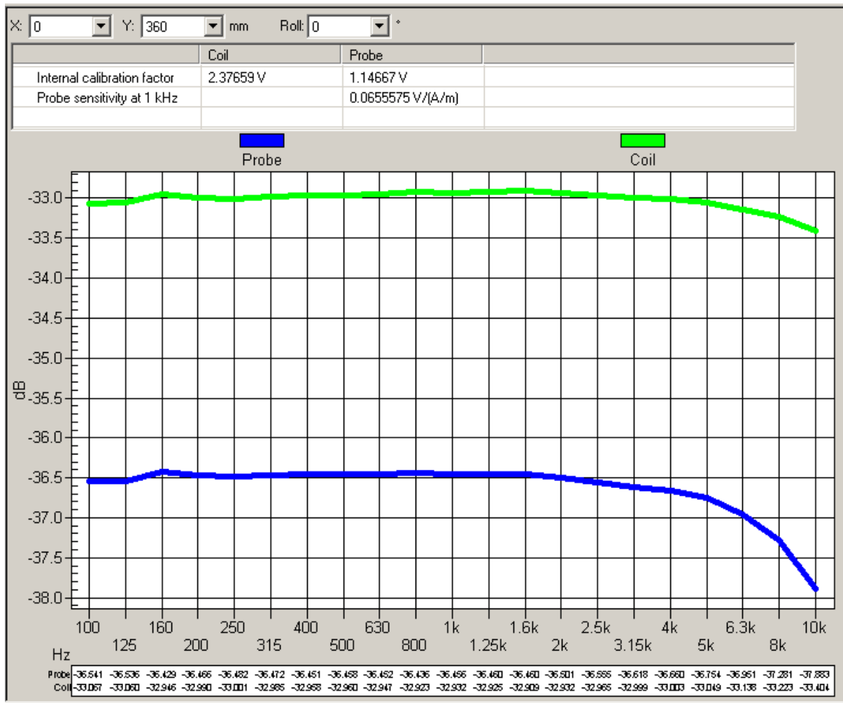
Graph 1: Frequency Response measured in AMCC
