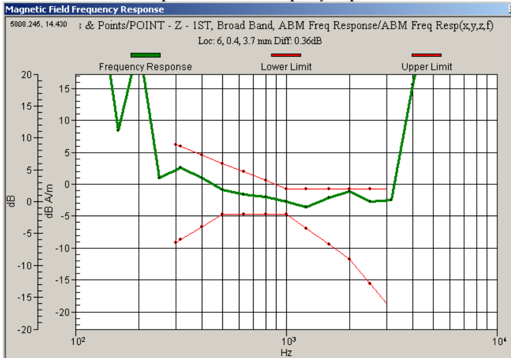
Graph 3: CDMA 1900 Frequency Response
