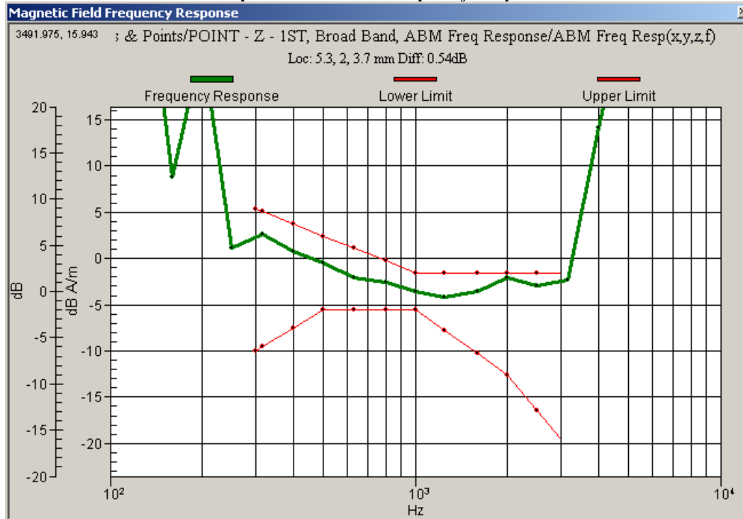
Graph 2: CDMA 800 Frequency Response
