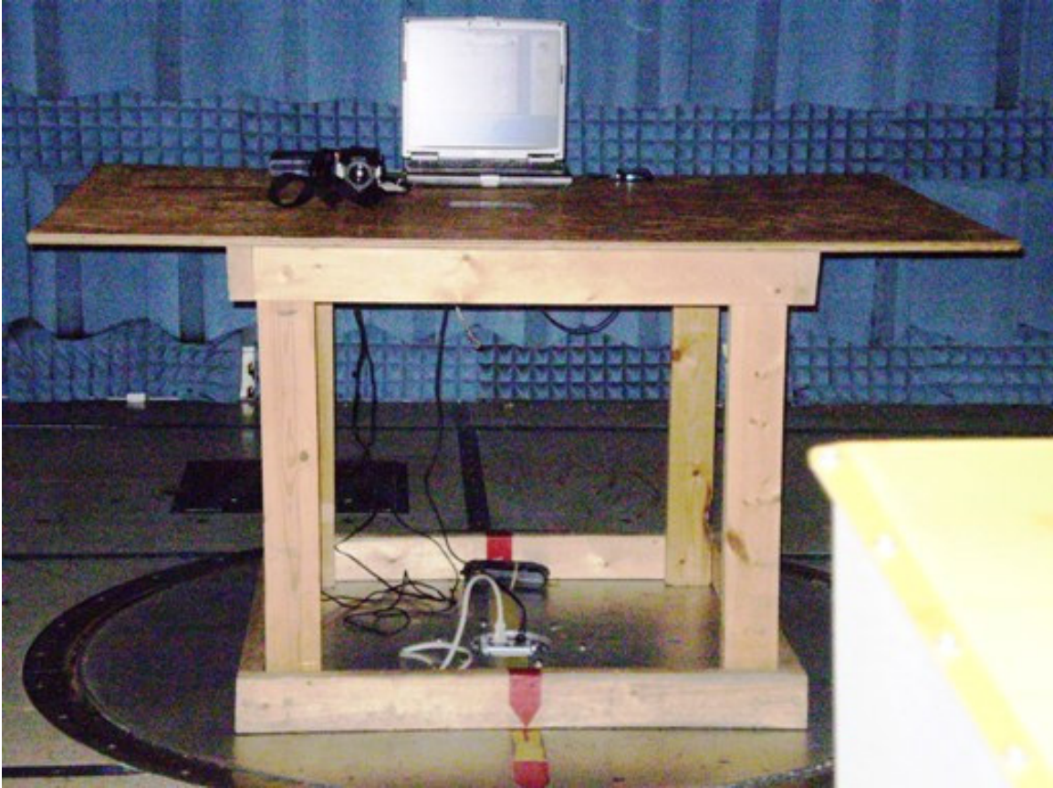
Part 15, PC Peripheral Radiated Emissions
