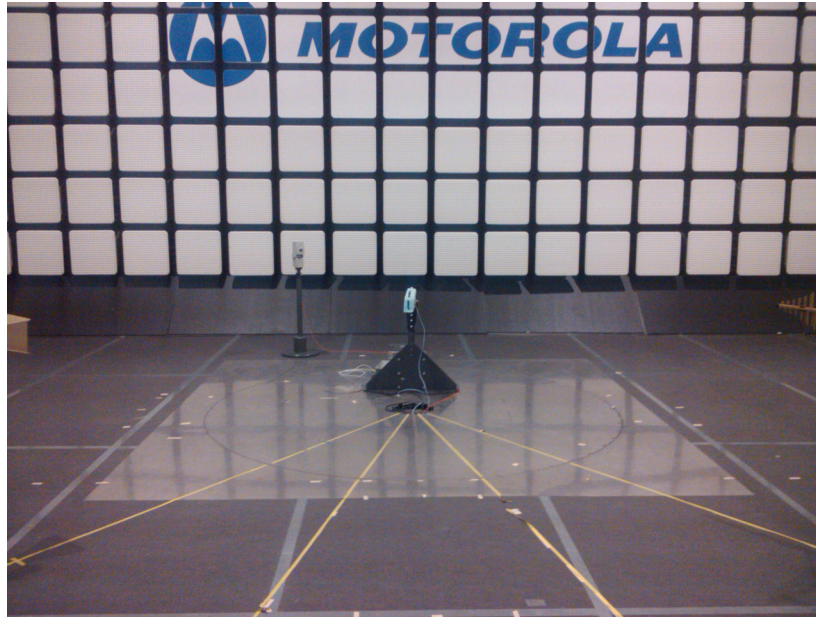
Radiated Emissions
