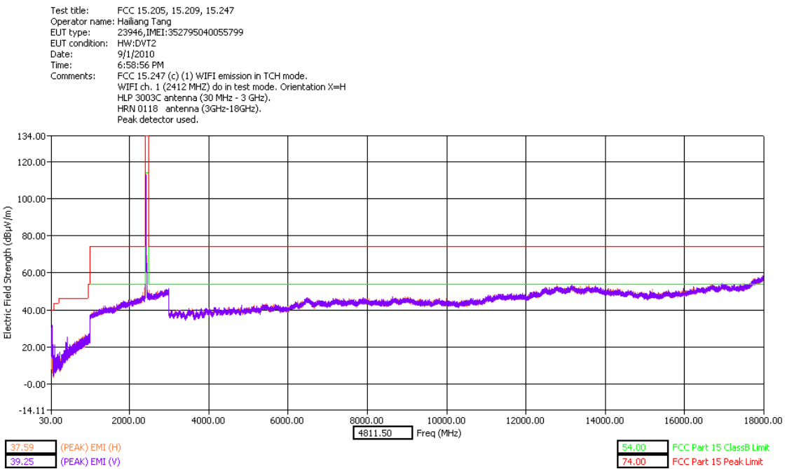
30 - 18000MHz Low Channel Dual Polarization X-Close
