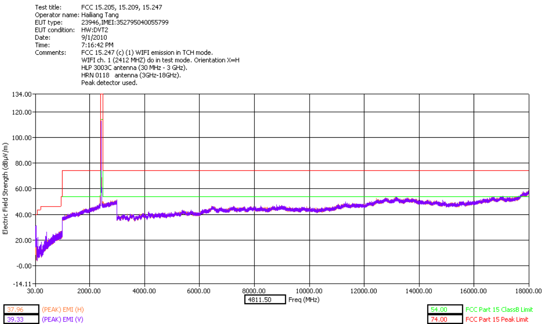
30 - 18000MHz Low Channel Dual Polarization X-Open
