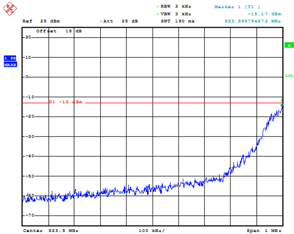
(Plot A5: GSM 850MHz Channel = 128)
