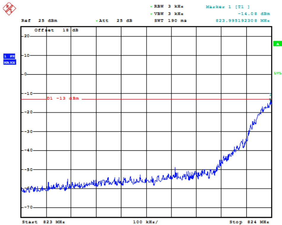
(Plot E5: GPRS 850MHz Channel = 128)
