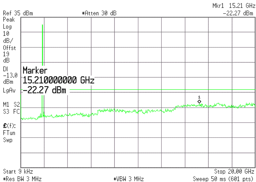
(Plot F4.: GSM 1900MHz Channel = 810, 9KHz to 20GHz)
