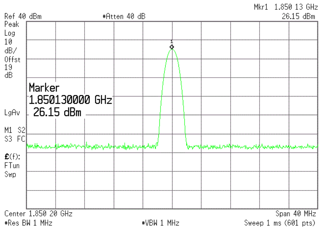
(Plot K1: EGPRS 1900MHz Channel = 512)
