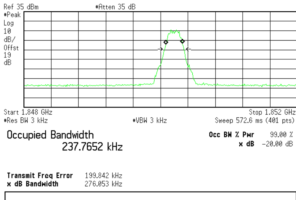
(Plot D3.2: EGPRS 1900MHz Channel = 512)
