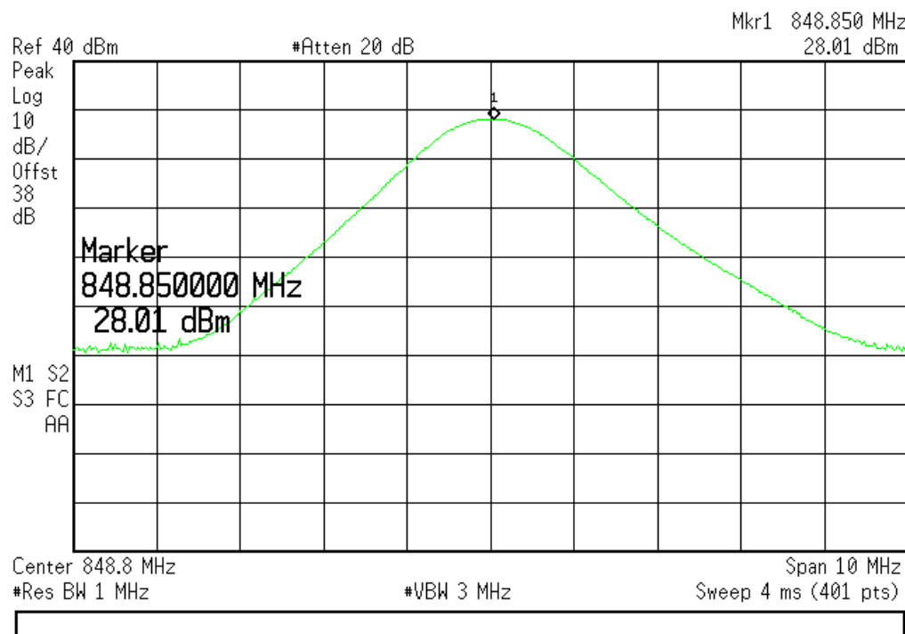
(Plot C6.1:GPRS 850MHz Channel = 251)
