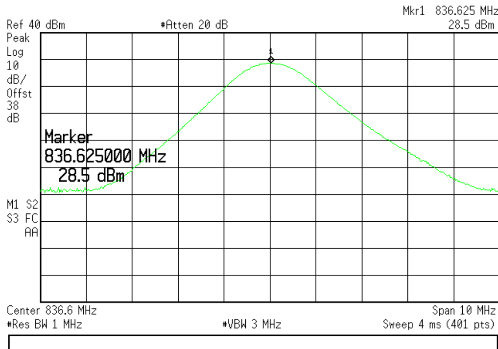
(Plot B6.1:GPRS 850MHz Channel = 190)
