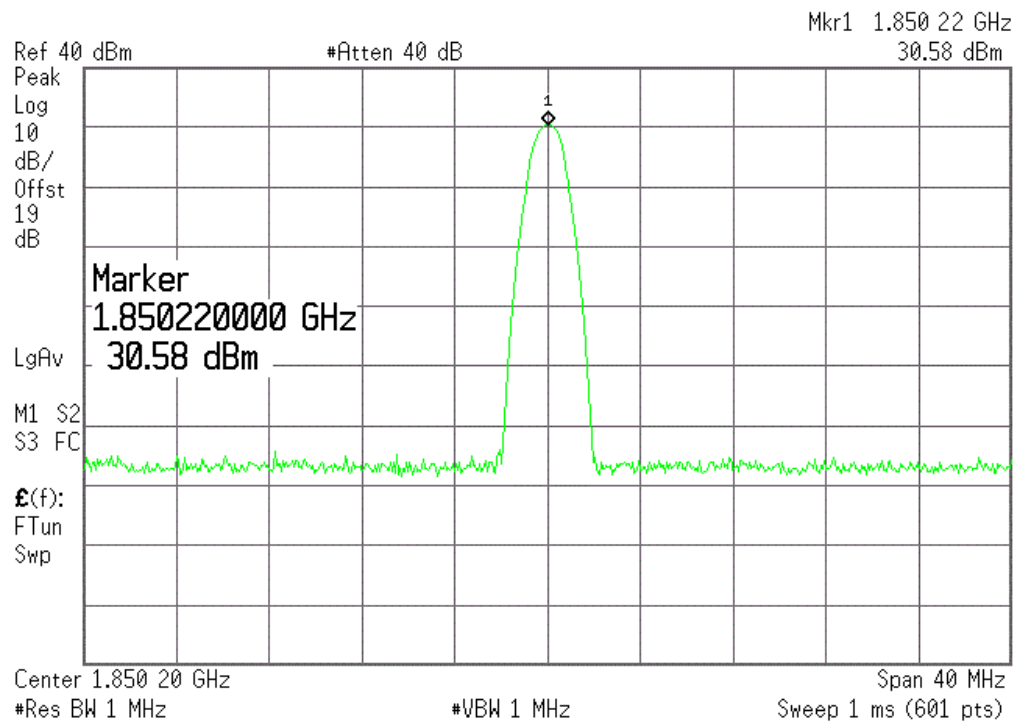
(Plot G1: GPRS 1900MHz Channel = 512)
