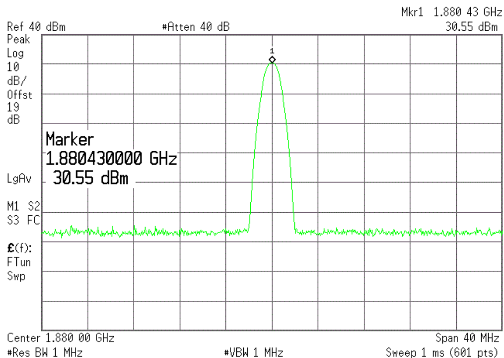
(Plot K2: GPRS 1900MHz Channel = 661)
