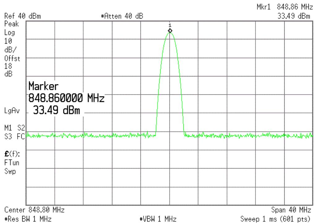
(Plot B1: GSM 850MHz Channel = 251)
