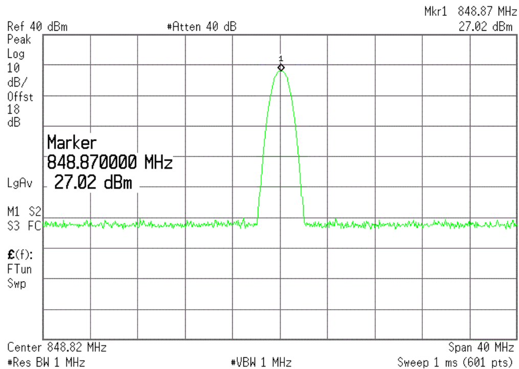
(Plot J1: EGPRS 850MHz Channel = 251)
