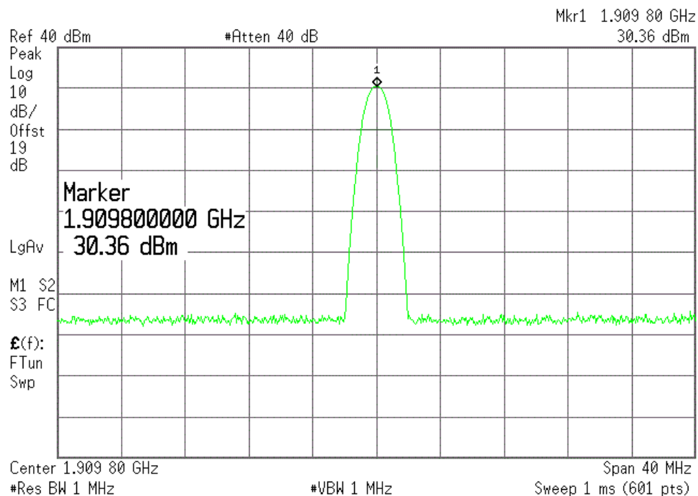
(Plot H1: GPRS 1900MHz Channel = 810)
