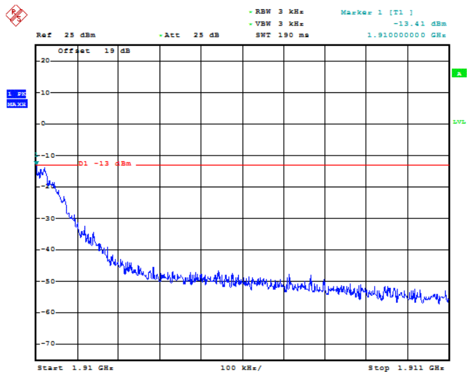
(Plot D5: GSM 1900MHz Channel = 810)
