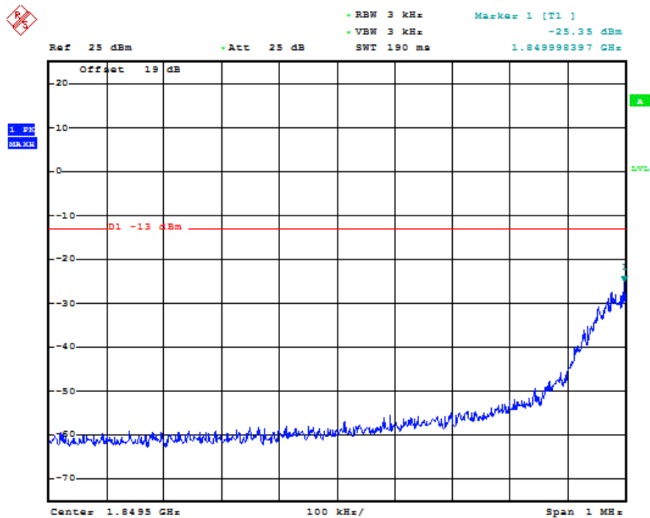
(Plot K5: EGPRS 1900MHz Channel = 512)
