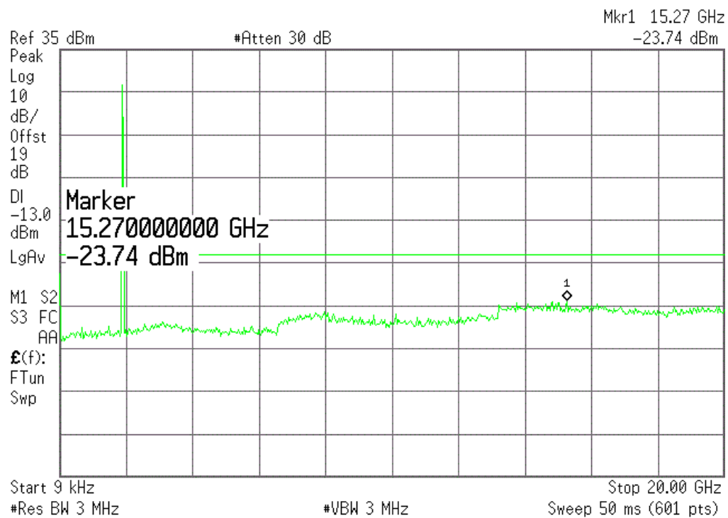
(Plot Q4.:EGPRS 1900MHz Channel = 661, 9KHz to 20GHz)
