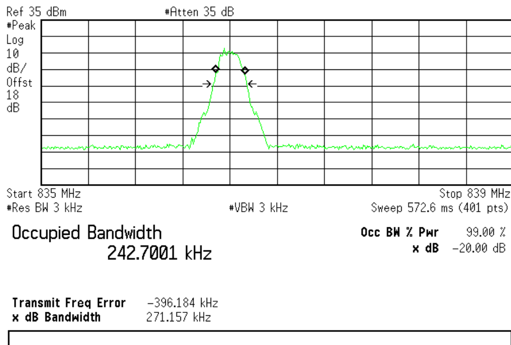
(Plot B3.2: EGPRS 850MHz Channel = 190)
