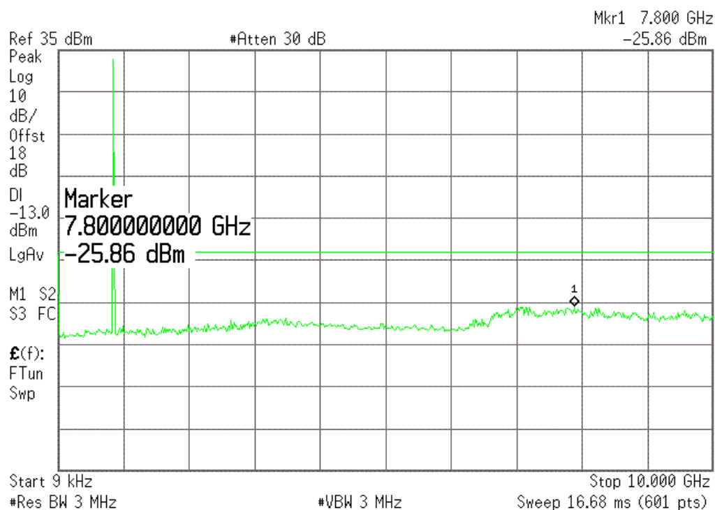
(Plot A4.:GSM 850MHz Channel = 128, 9KHz to 10GHz)
