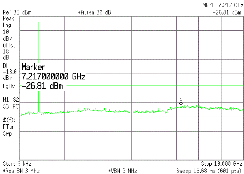
(Plot I4.: GPRS 850MHz Channel = 251, 9KHz to 10GHz)
