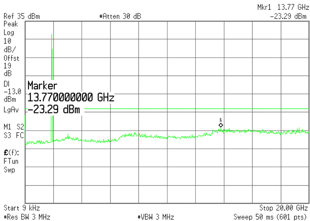
(Plot K4.: GPRS 1900MHz Channel = 661, 9KHz to 20GHz)
