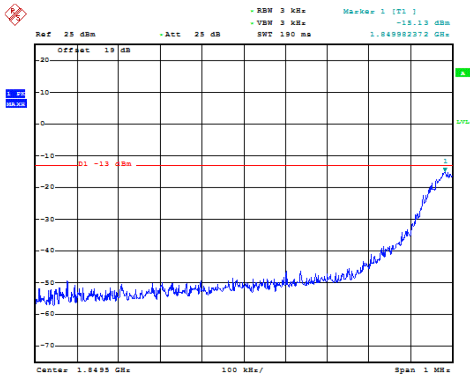
(Plot G5: GPRS 1900MHz Channel = 512)
