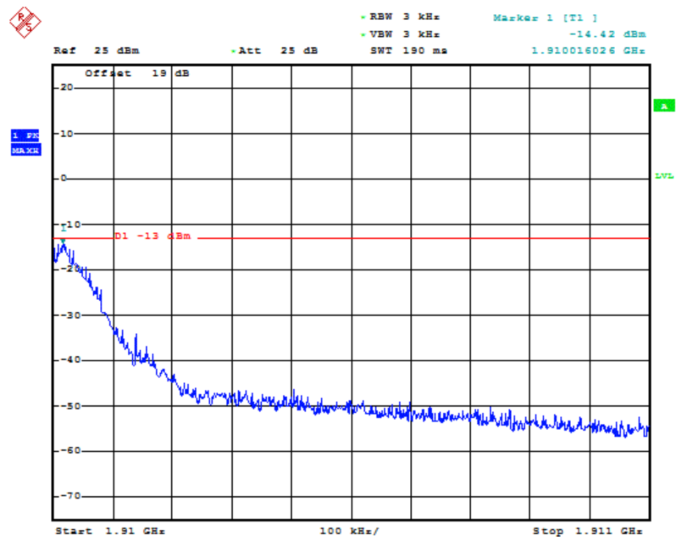
(Plot H5: GPRS 1900MHz Channel = 810)
