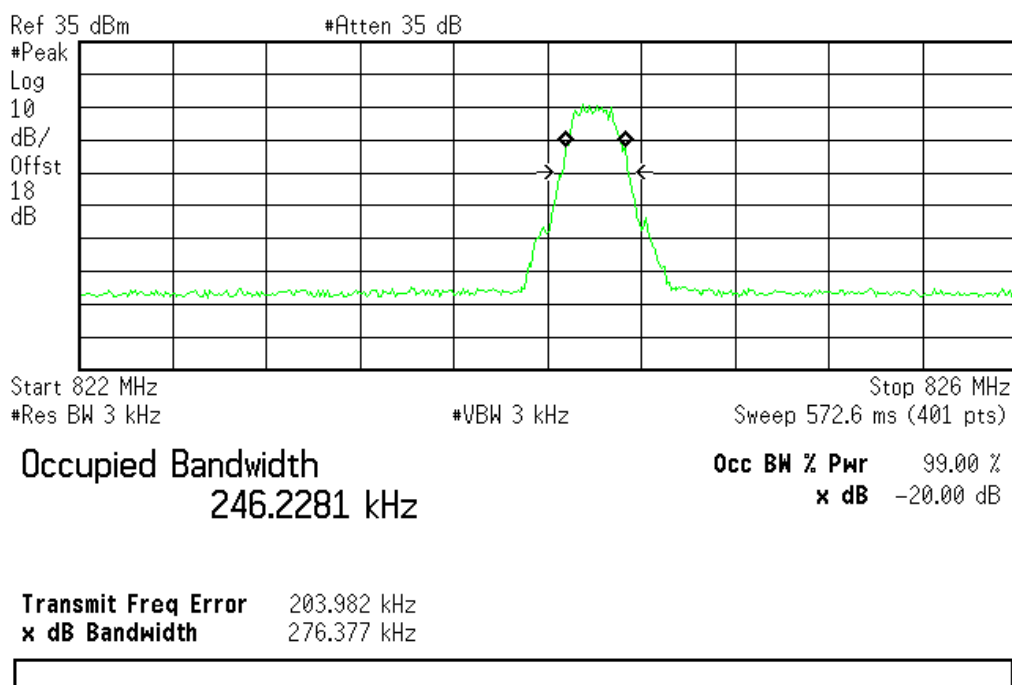
(Plot A3.2: EGPRS 850MHz Channel = 128)
