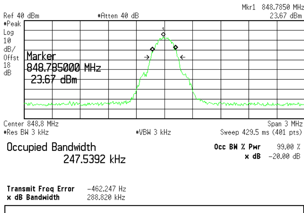
(Plot C3.1: GPRS 850MHz Channel = 251)
