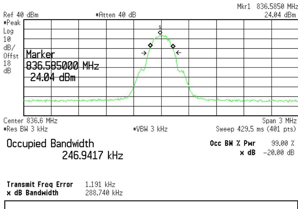
(Plot B3.1: GPRS 850MHz Channel = 190)
