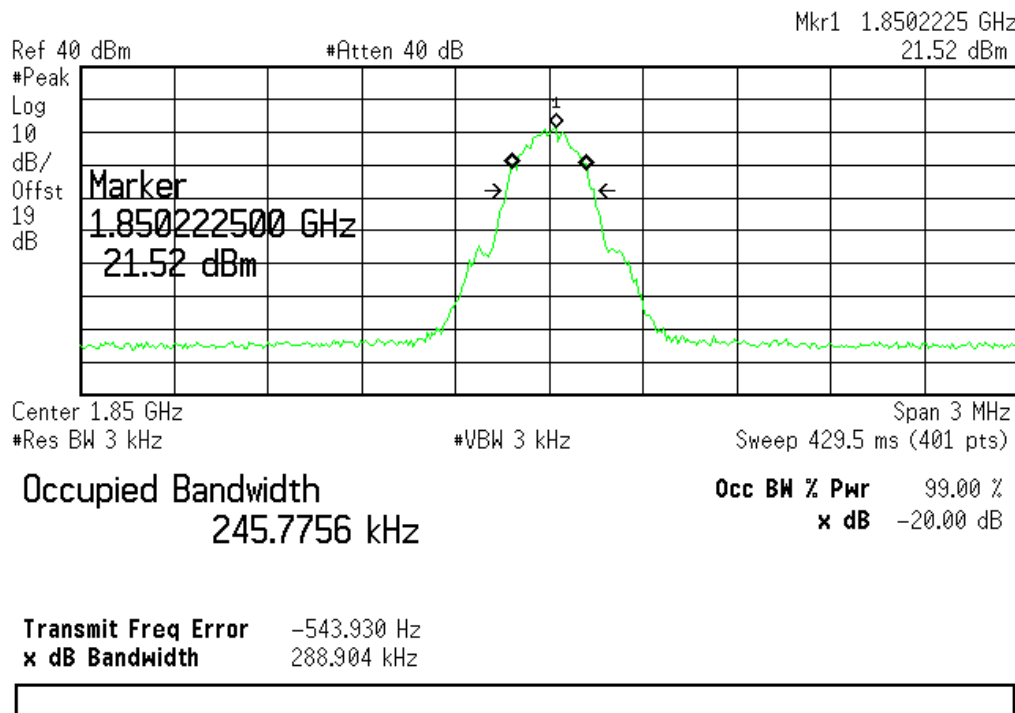
(Plot D3.1: GPRS 1900MHz Channel = 512)
