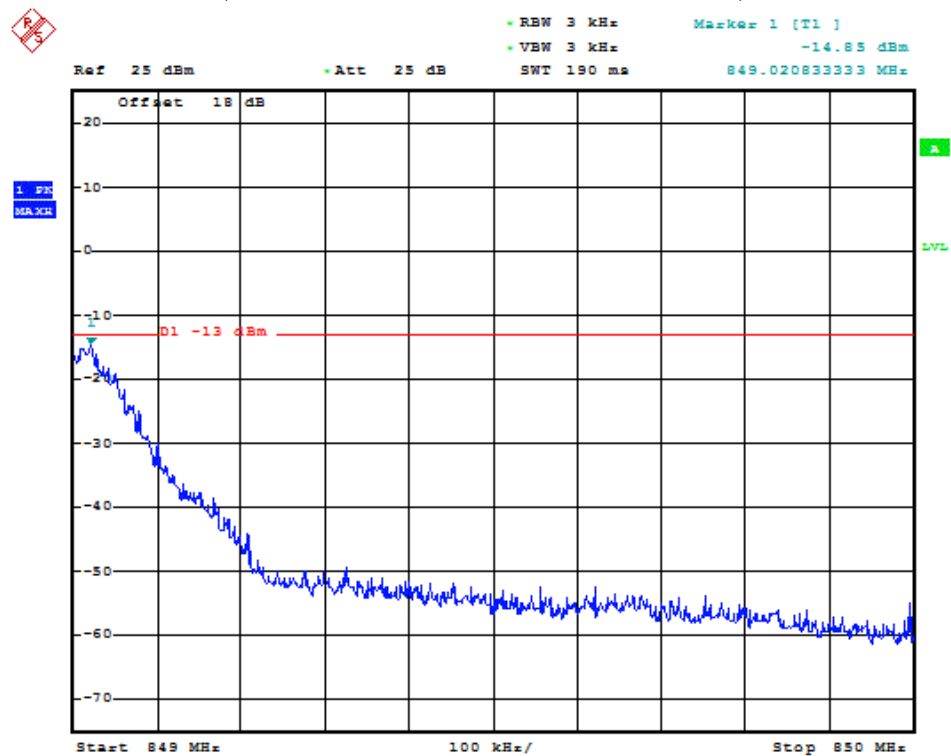
(Plot F5: GPRS 850MHz Channel = 251)
