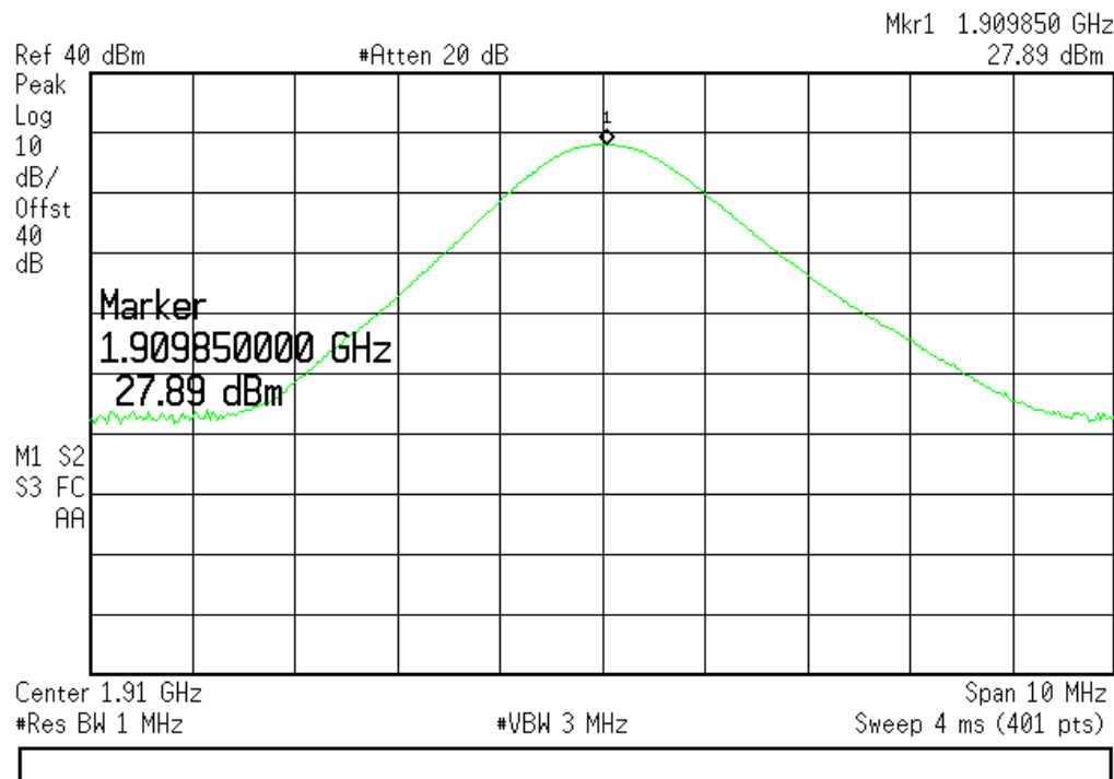
(Plot F6.1:GPRS 1900MHz Channel = 810)
