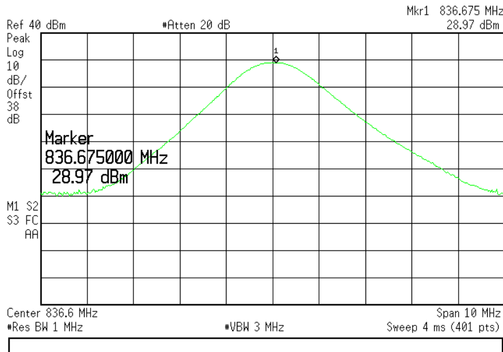
(Plot B6:GSM 850MHz Channel = 190)
