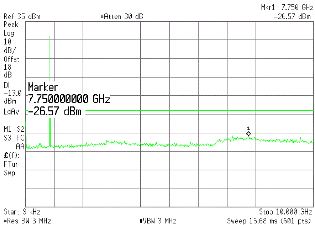
(Plot M4.:EGPRS 850MHz Channel = 128, 9KHz to 10GHz)
