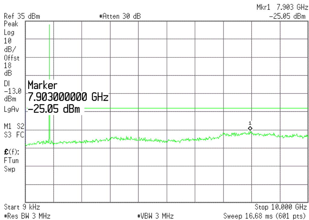
(Plot C4.:GSM 850MHz Channel = 251, 9KHz to 10GHz)
