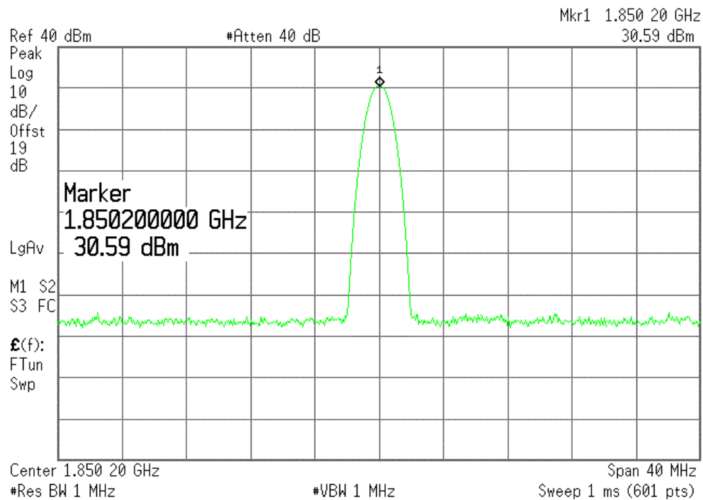
(Plot C1: GSM 1900MHz Channel = 512)
