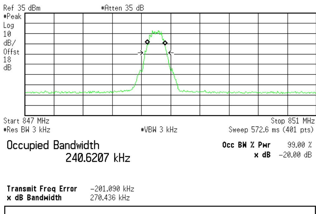
(Plot C3.2: EGPRS 850MHz Channel = 251)
