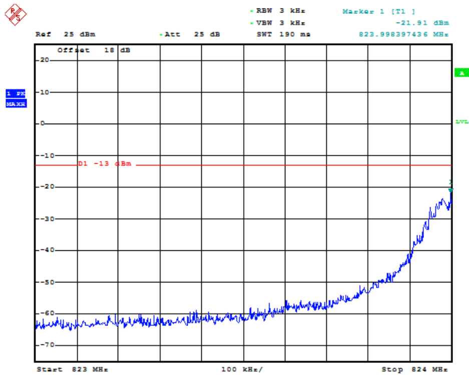
(Plot I5: EGPRS 850MHz Channel = 128)
