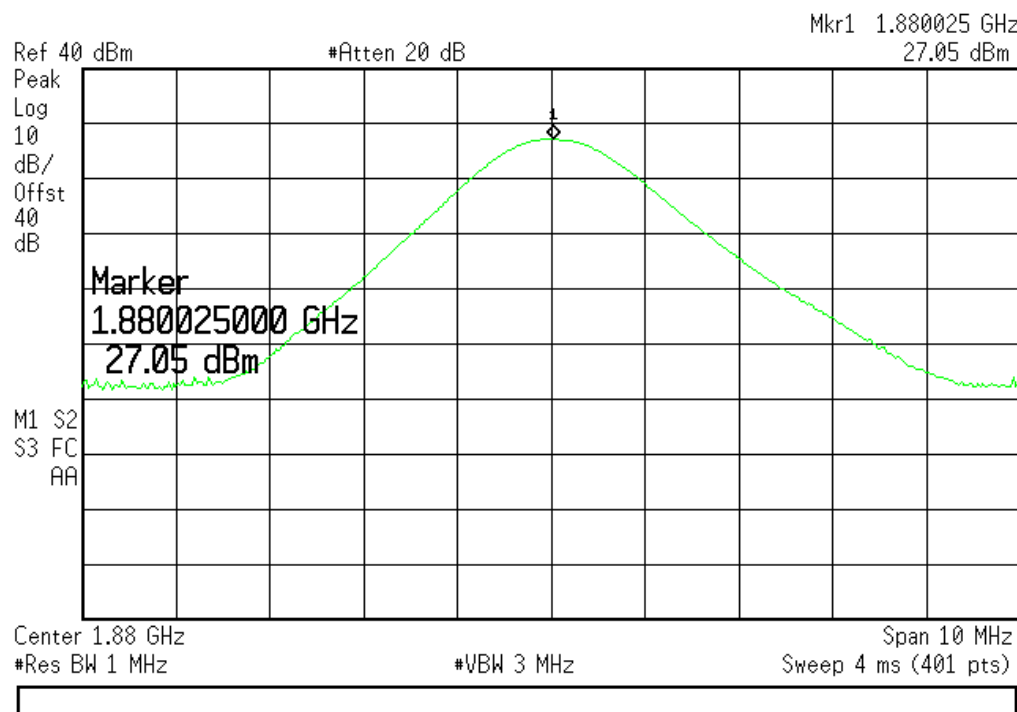
(Plot E6.1:GPRS 1900MHz Channel = 661)
