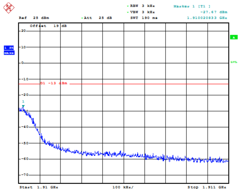
(Plot L5: EGPRS 1900MHz Channel = 810)
