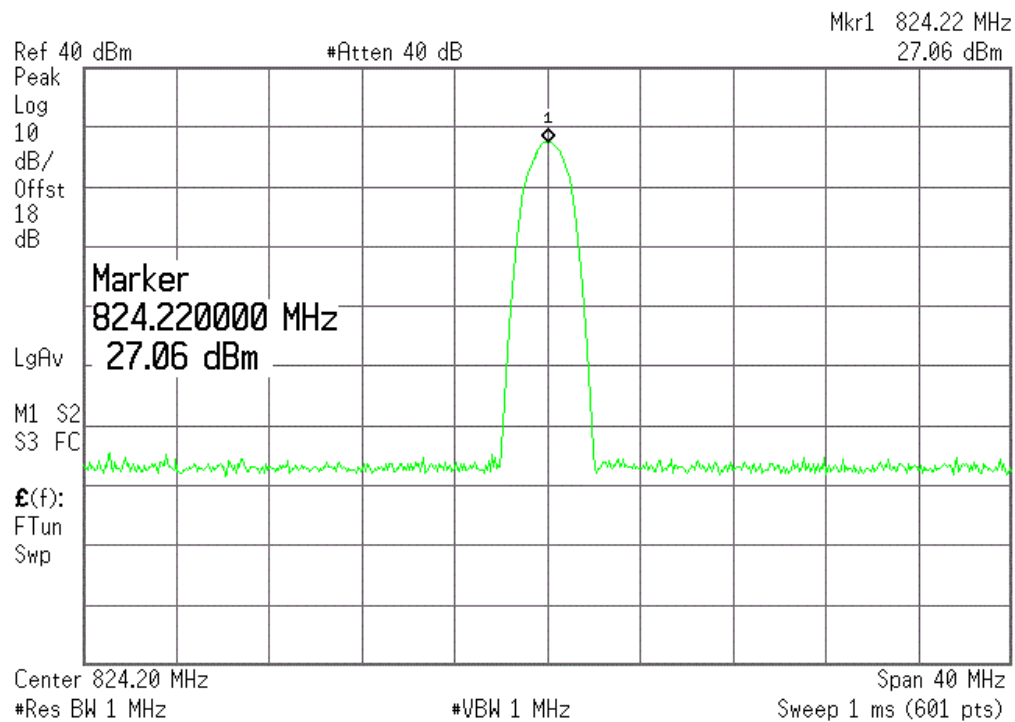
(Plot I1: EGPRS 850MHz Channel = 128)
