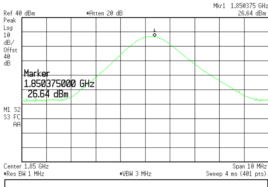
(Plot D6.1:GPRS 1900MHz Channel = 512)
