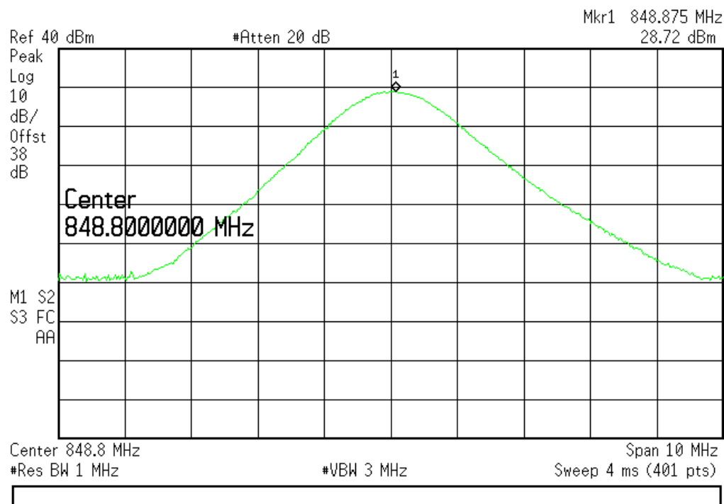
(Plot C6:GSM 850MHz Channel = 251)
