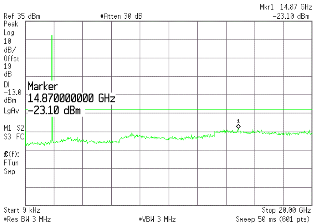
(Plot J4.: GPRS 1900MHz Channel = 512, 9KHz to 20GHz)
