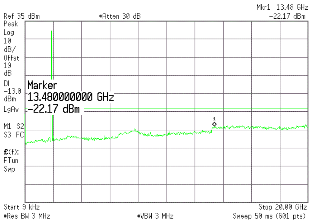
(Plot E4.: GSM 1900MHz Channel = 661, 9KHz to 20GHz)
