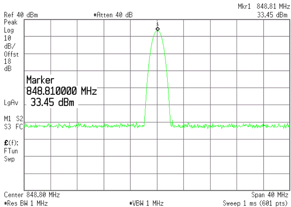
(Plot F1: GPRS 850MHz Channel = 251)
