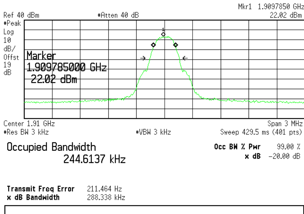
(Plot F3.1: GPRS 1900MHz Channel = 810)
