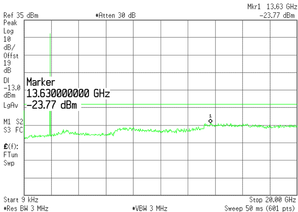
(Plot L4.: GPRS 1900MHz Channel = 810, 9KHz to 20GHz)
