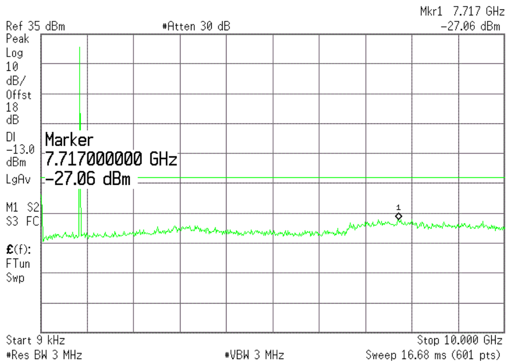
(Plot H4.: GPRS 850MHz Channel = 190, 9KHz to 10GHz)
