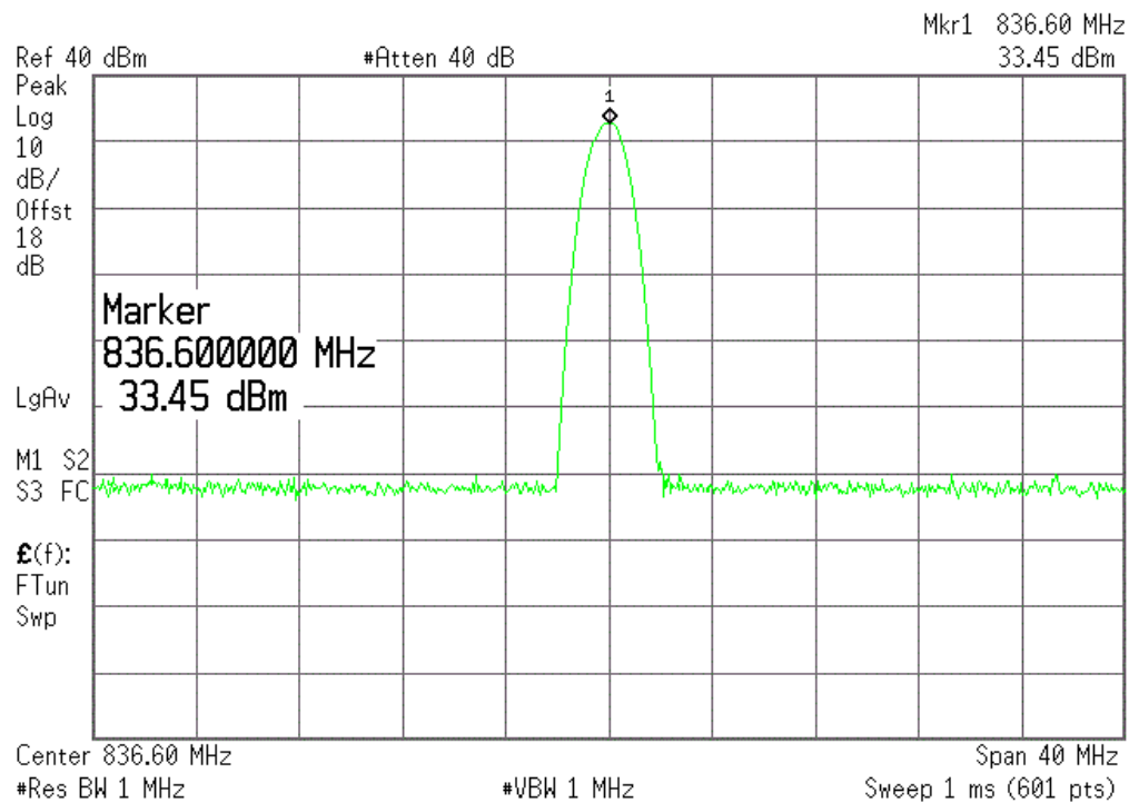
(Plot H2: GPRS 850MHz Channel = 190)
