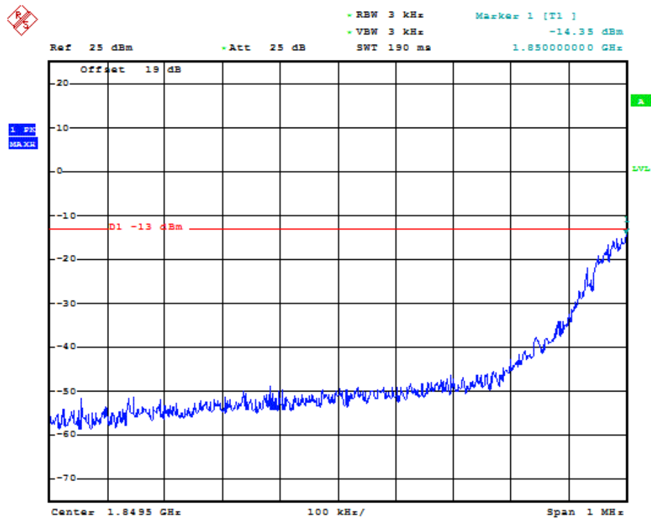
(Plot C5: GSM 1900MHz Channel = 512)
