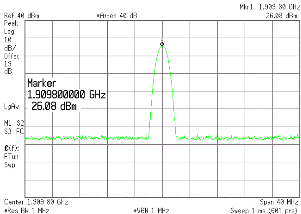
(Plot L1: EGPRS 1900MHz Channel = 810)
