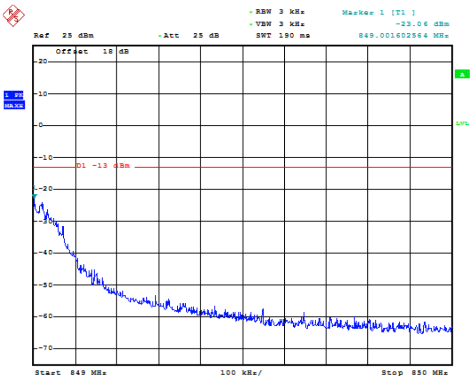
(Plot J5: EGPRS 850MHz Channel = 251)
