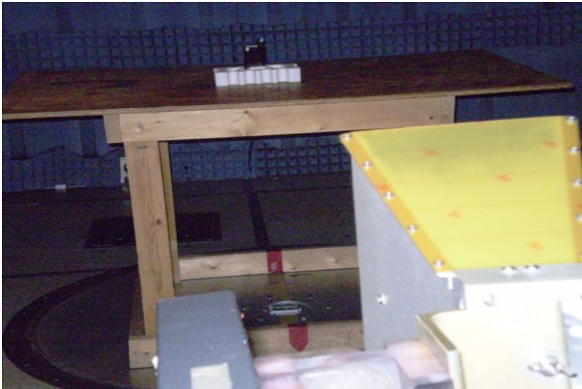
Radiated Emissions
