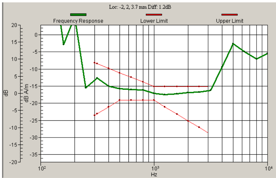
Graph 5: WCDMA 1700 Frequency Response
