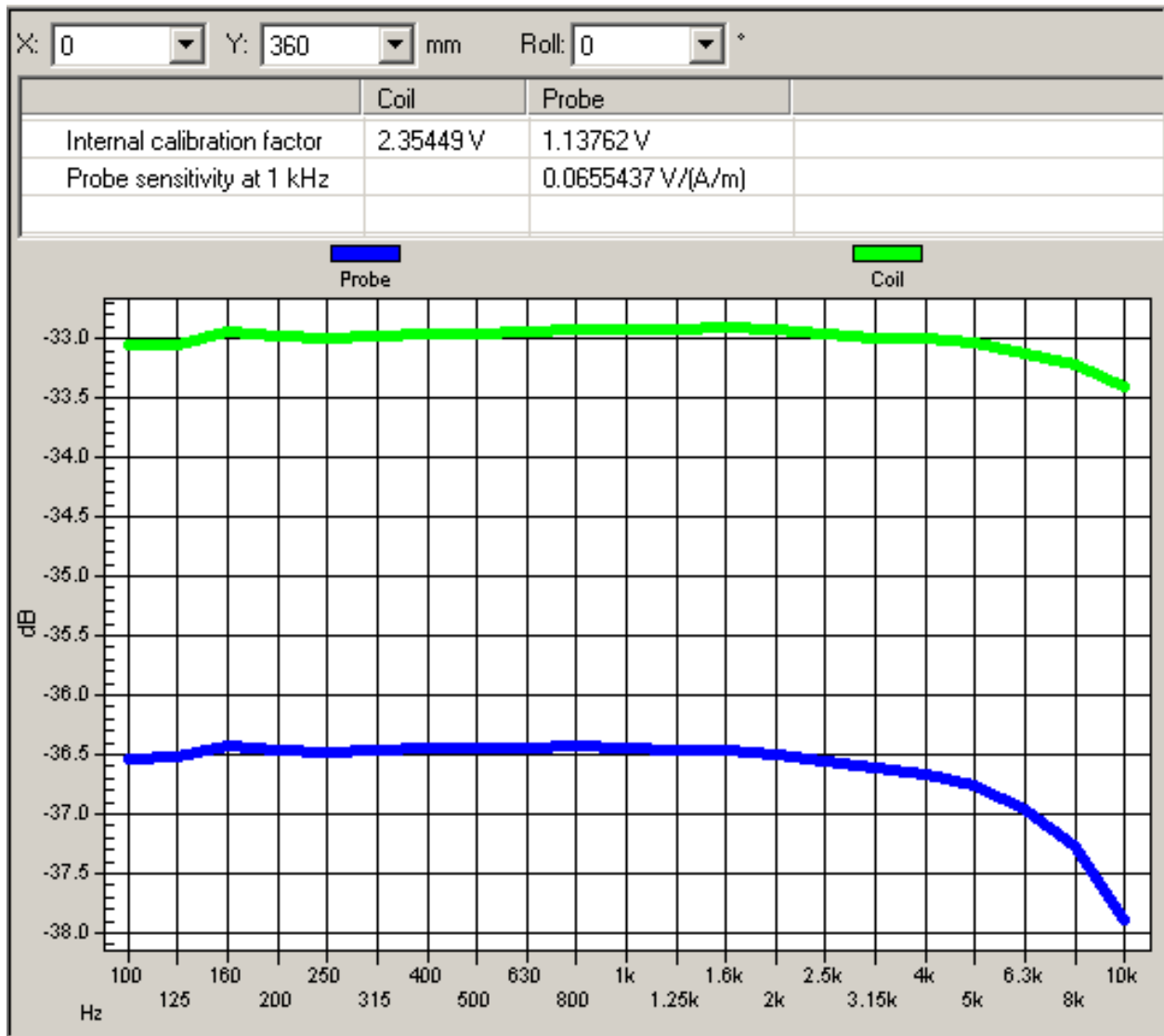
Graph 1: Frequency Response measured in AMCC
