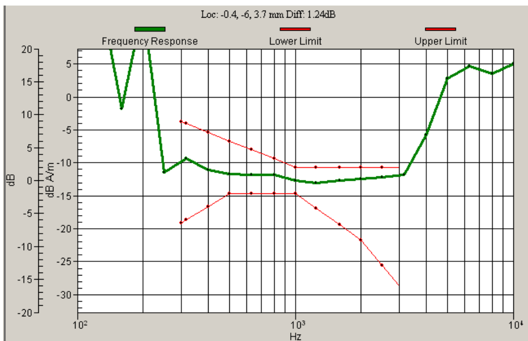
Graph 2: GSM 850 Frequency Response
