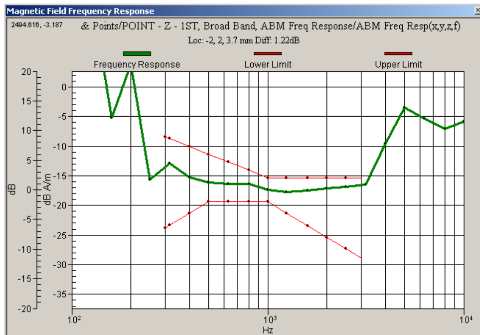
Graph 3: WCDMA 850 Frequency Response
