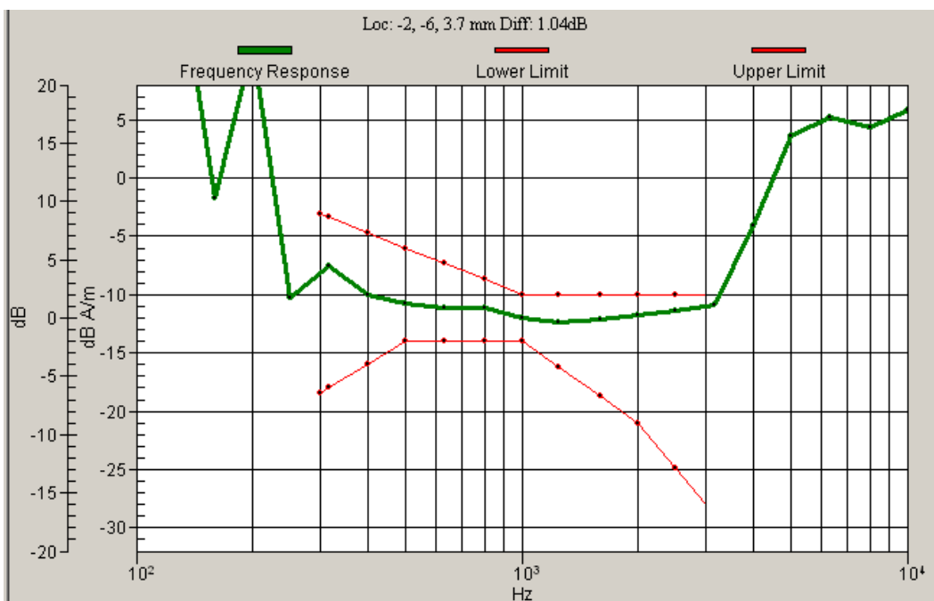
Graph 3: GSM 1900 Frequency Response
