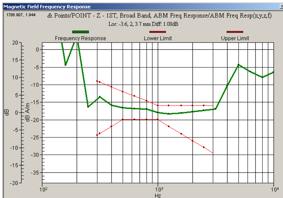
Graph 4: WCDMA 1900 Frequency Response
