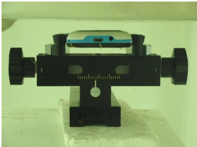
Rear Face of the DUT with Phantom 1 cm Gap (EUT without Earphone)
