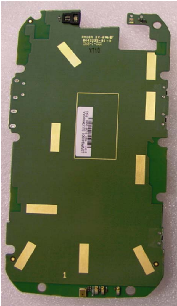
Main Board Front (No Shields placed on this side)
