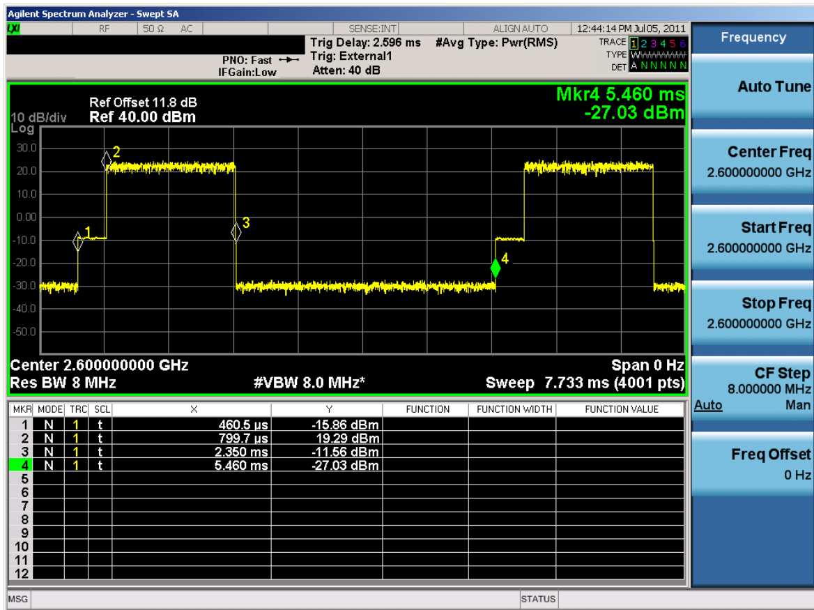
Figure 14-2 Timing Plot for WIMAX Signal – PUSC
