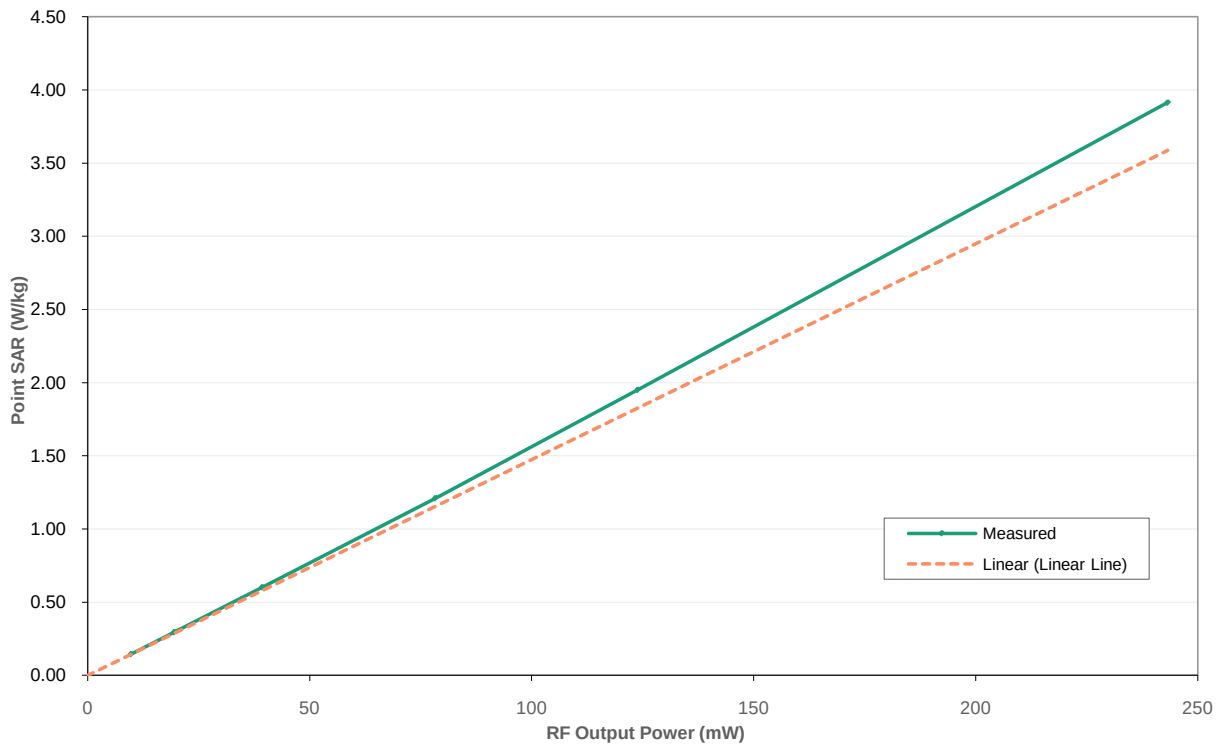
AMC, 5 MHz, QPSK, Tx 2
