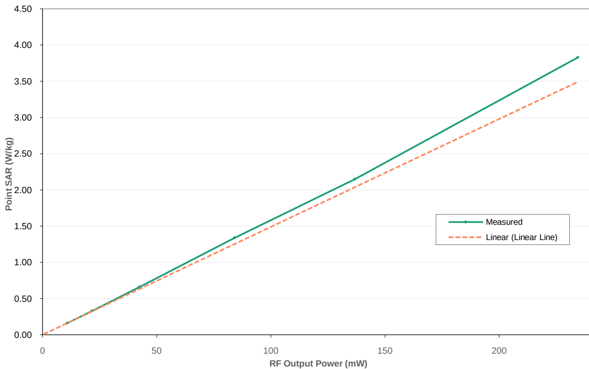
AMC, 10 MHz, QPSK, Tx 2
