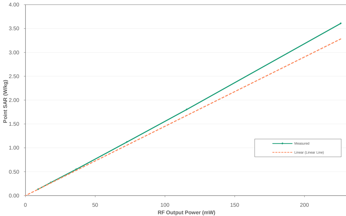
PUSC, 5 MHz, QPSK, Tx 2
