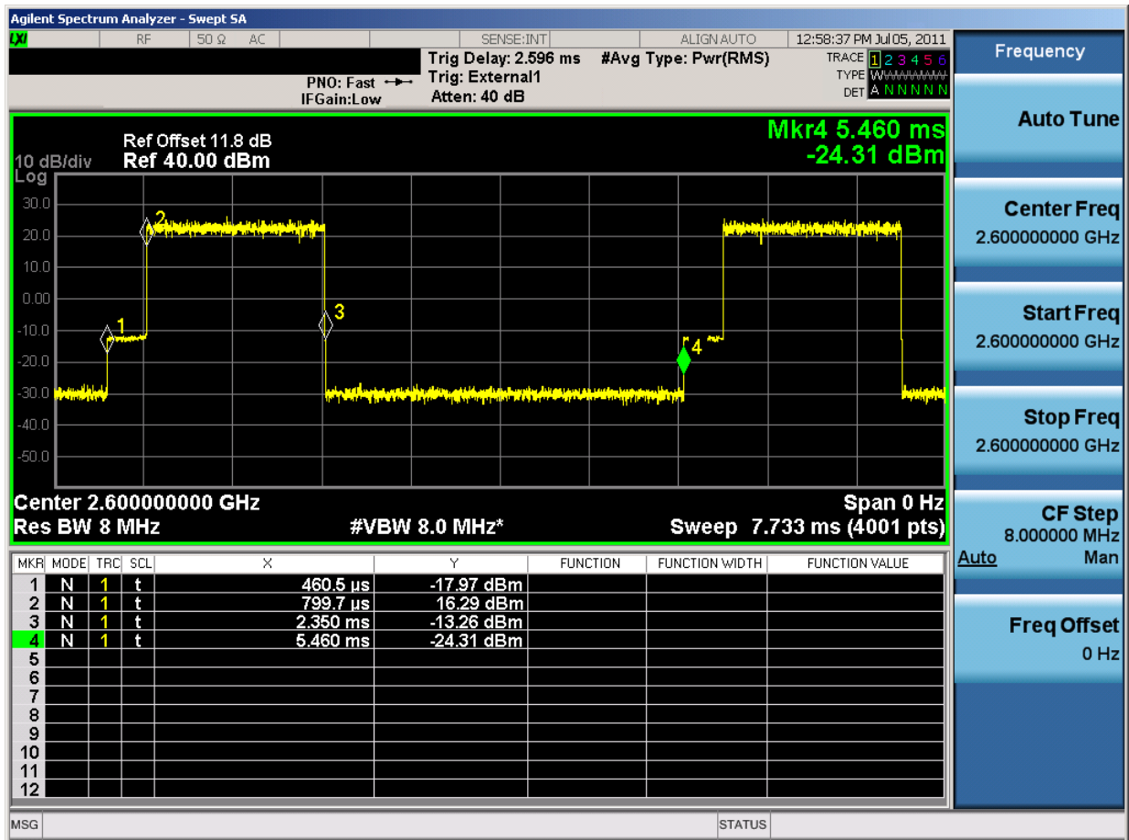
Figure 14-3 Timing Plot for WIMAX Signal – BAMC
