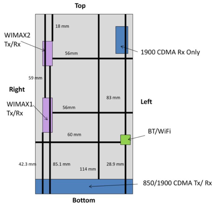
Figure 15-1 Identification of Sides for SAR Testing (Back View)
