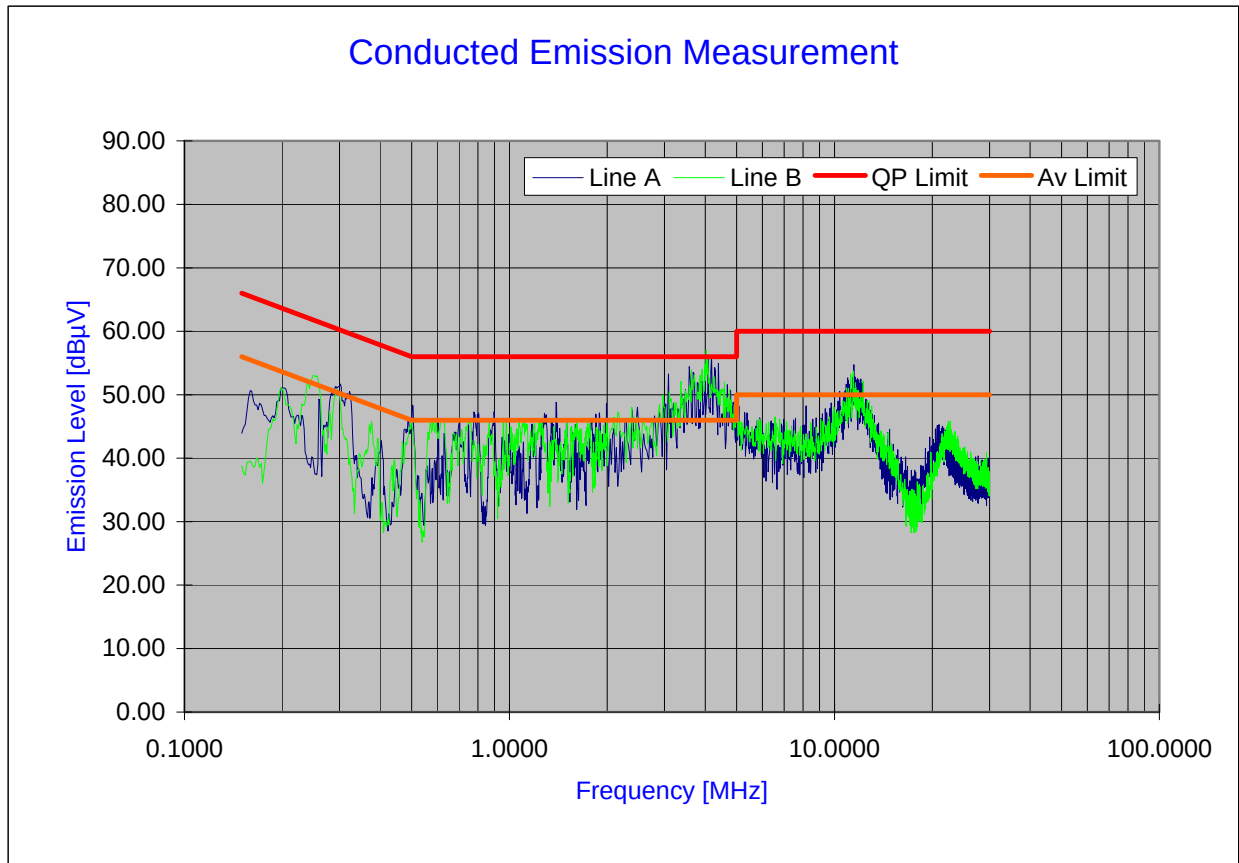
Plot 6-34. Line Conducted Plot with 802.11n (800ns)
