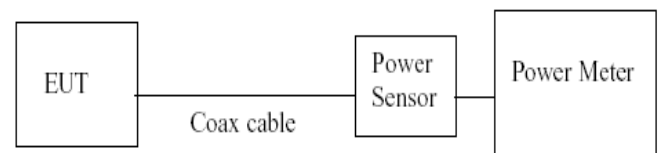
Figure 6-5. Test Instrument & Measurement Setup
