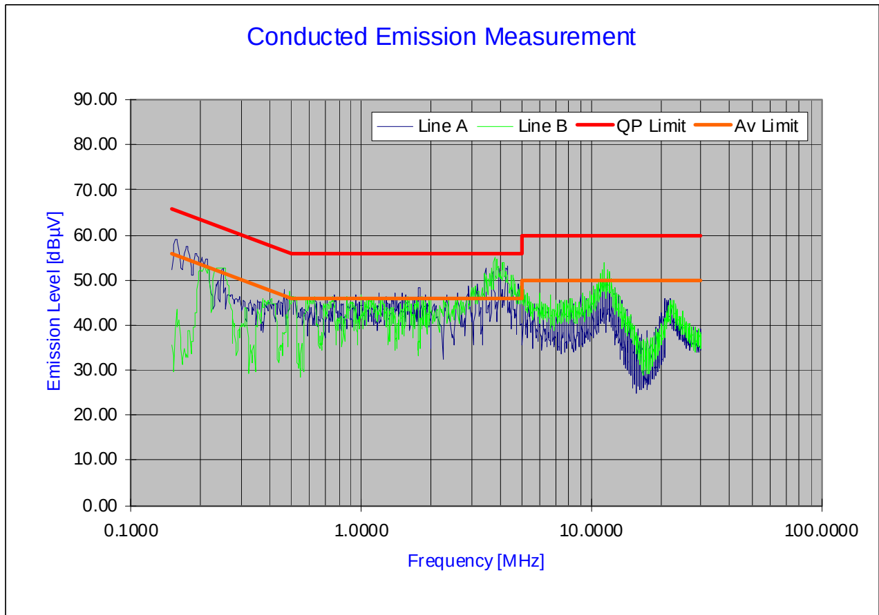
Plot 6-33. Line Conducted Plot with 802.11n (400ns)
