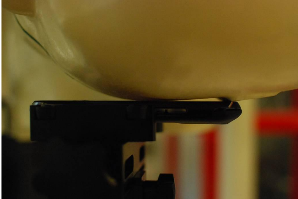
Figure 24-3 SAR Test Setup Photo – Left Touch
