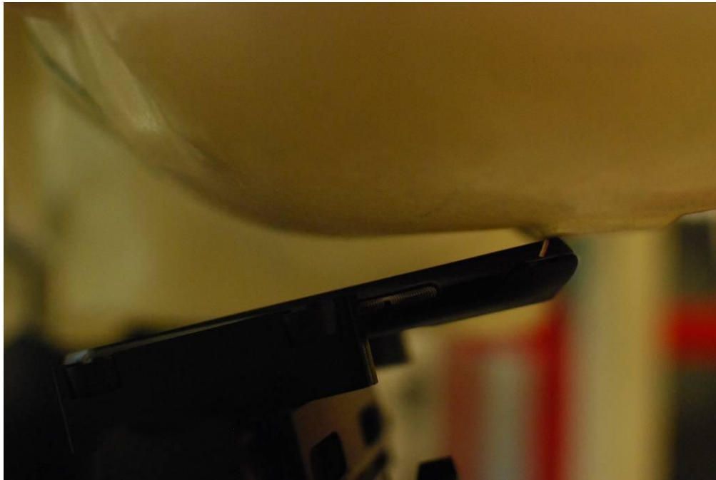
Figure 24-4 SAR Test Setup Photo – Left Tilt
