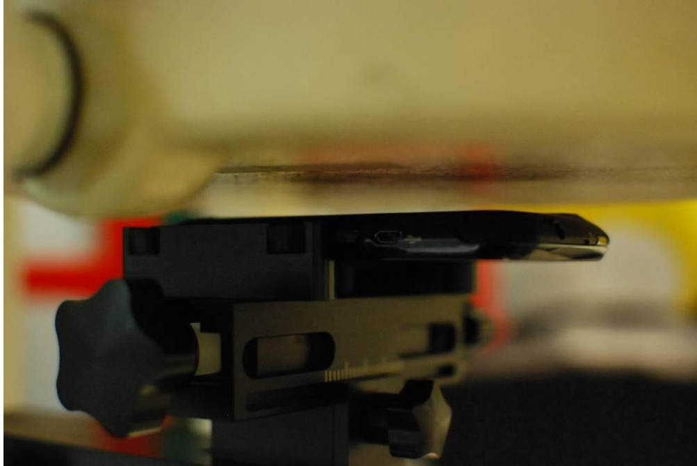
Figure 24-5 SAR Test Setup Photo – Back at 1.0 cm
