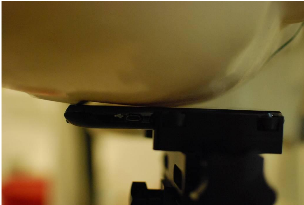
Figure 24-1 SAR Test Setup Photo – Right Touch
