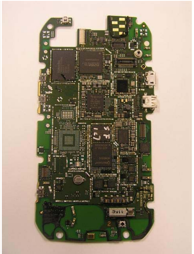
Main Board Back Without Shields
