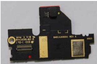
Daughter Board Top W/ Ground Plate
