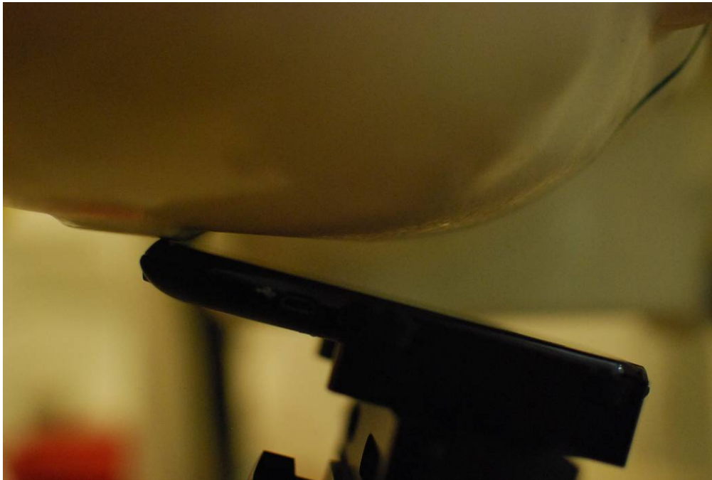
Figure 22-2 SAR Test Setup Photo – Right Tilt
