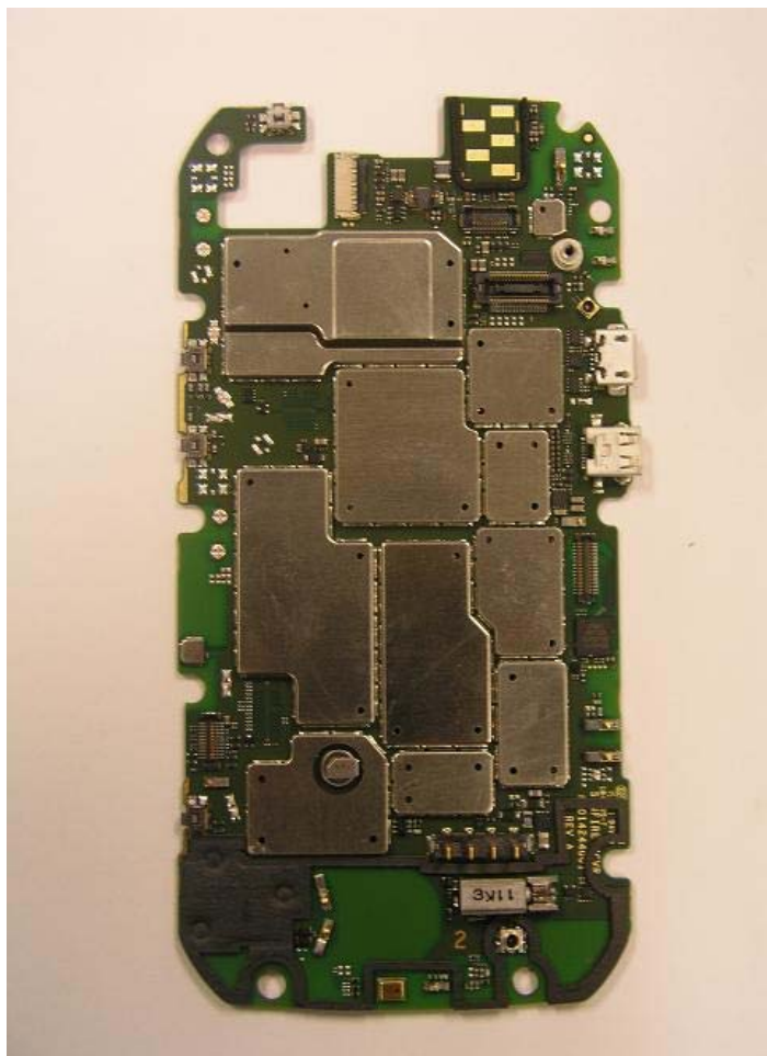
Main Board Back With Shields
