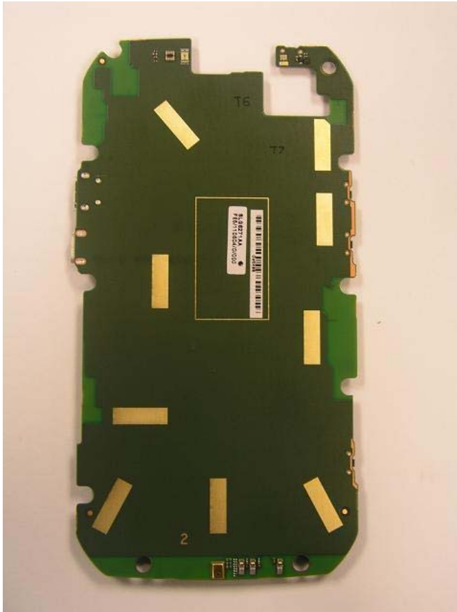
Main Board Front No shields placed on this side
