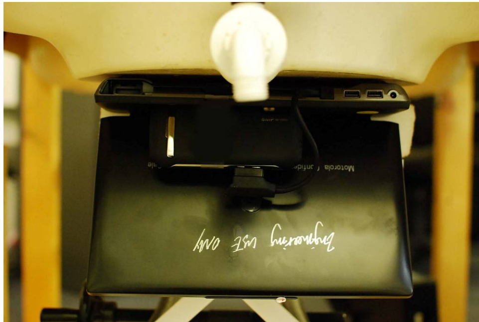
SAR Test Setup Photo 1 – Lapdock Front View
