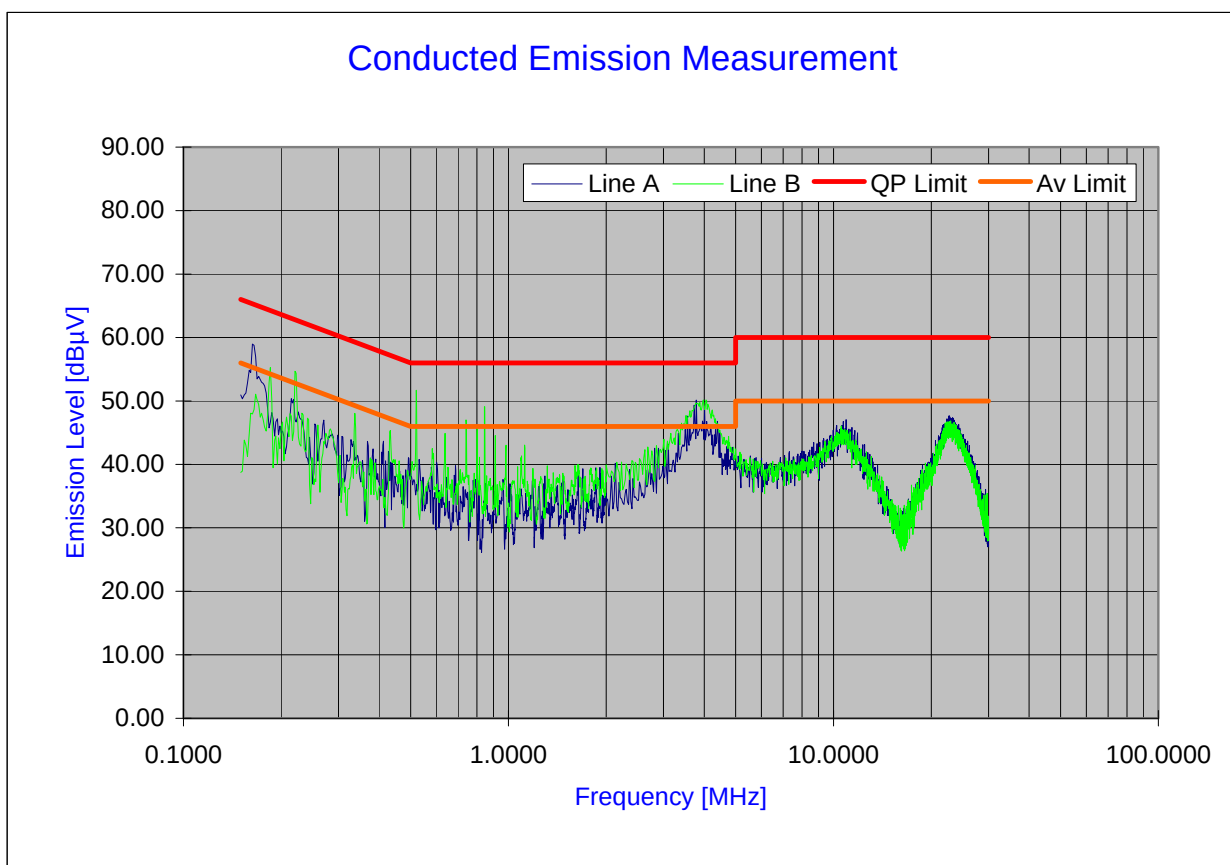
Plot 6-26. Line Conducted Plot with Bluetooth
