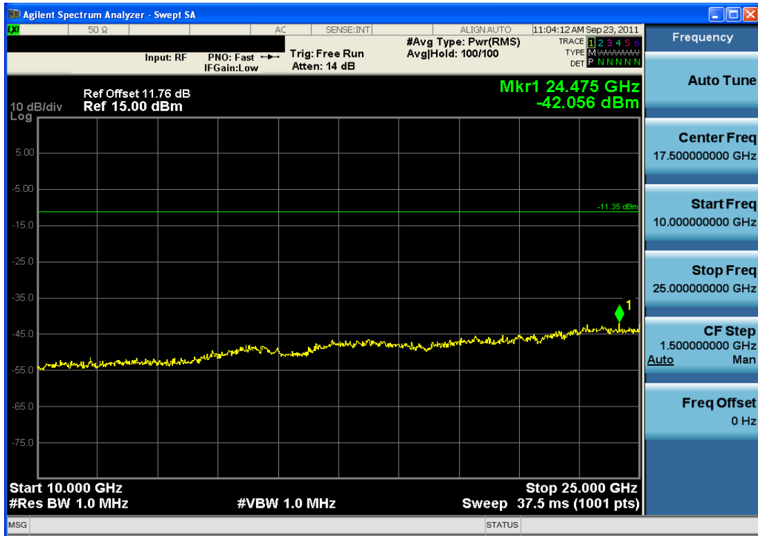
Plot 6-21. Conducted Spurious Plot (Bluetooth, 3Mbps – Ch. 0)
