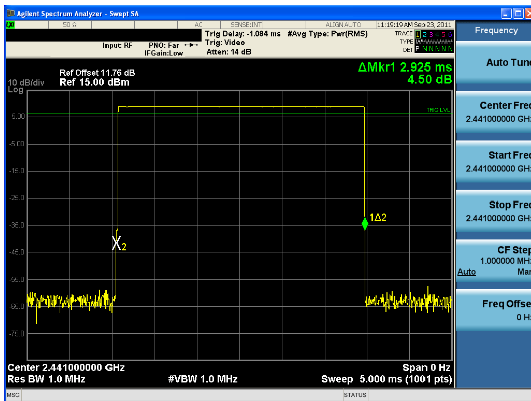
Plot 6-17. Time of Occupancy Plot (Standard Bluetooth Mode)
