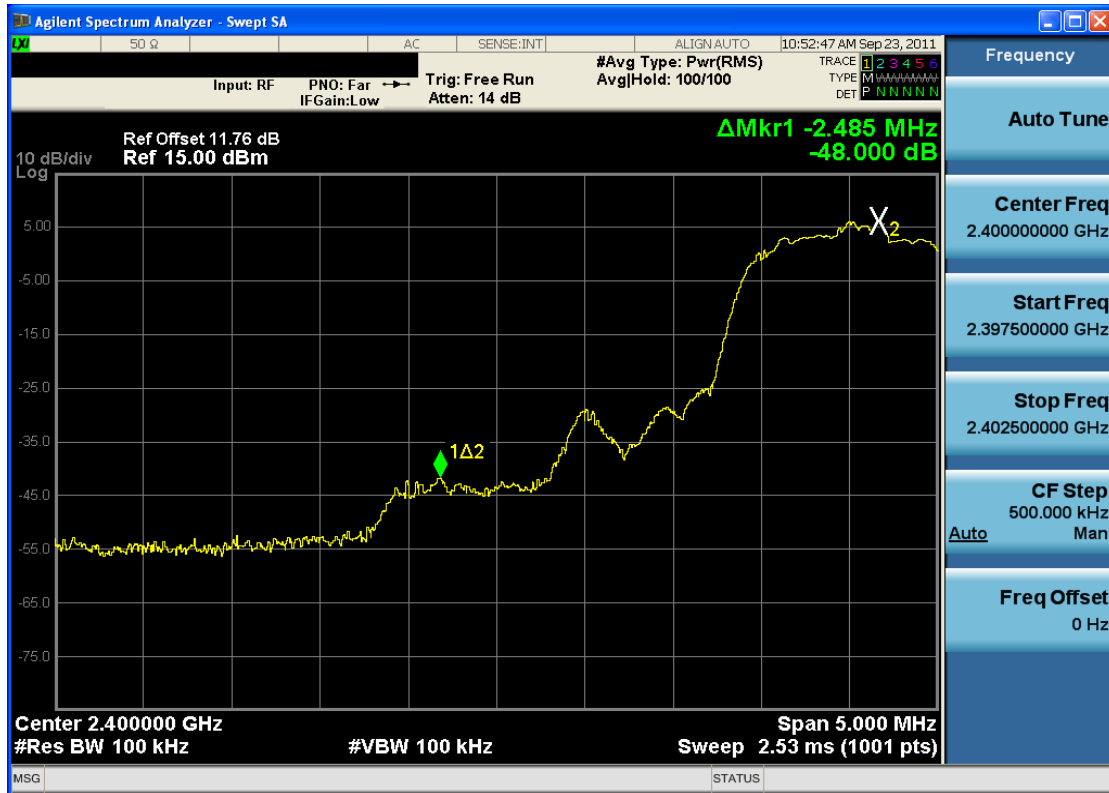
Plot 6-13. Band Edge Plot (Bluetooth, 3Mbps – Ch. 0)
