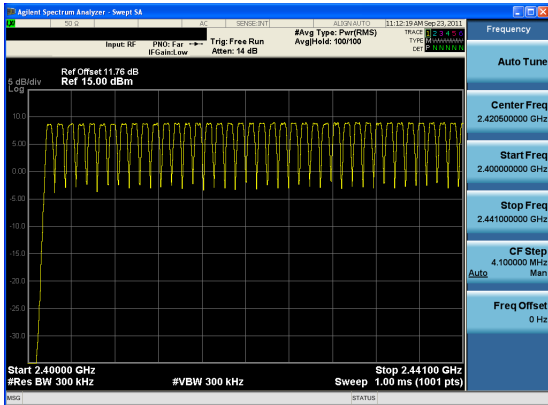
Plot 6-18. Low End Spectrum Channel Hopping Plot (Bluetooth)
