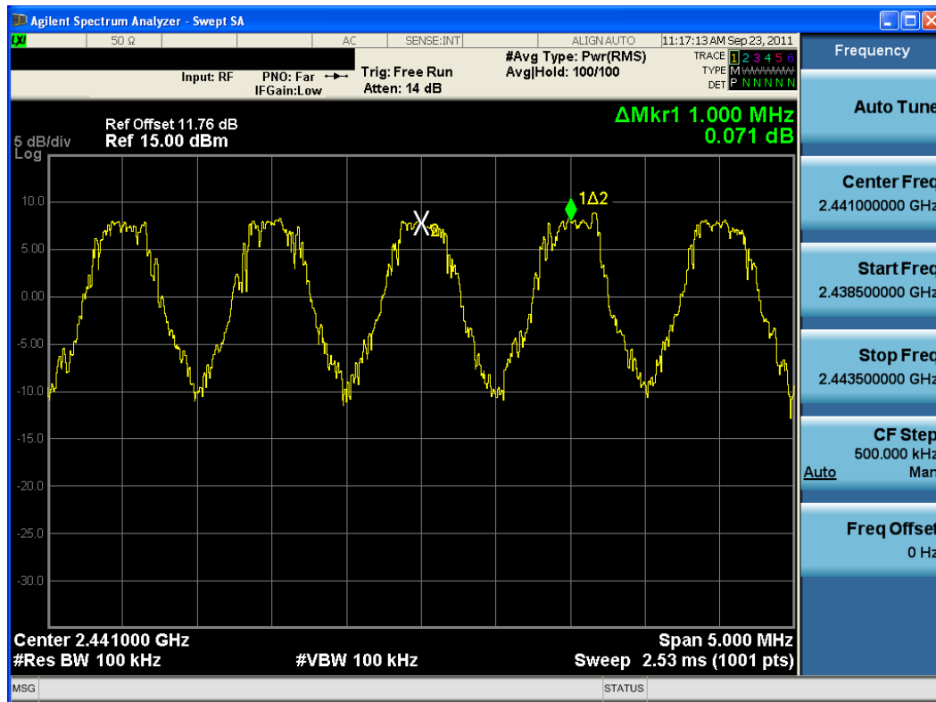
Plot 6-15. Channel Spacing Plot (Bluetooth)
