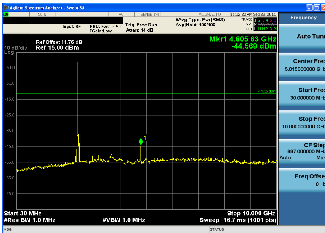
Plot 6-20. Conducted Spurious Plot (Bluetooth, 3Mbps – Ch. 0)
