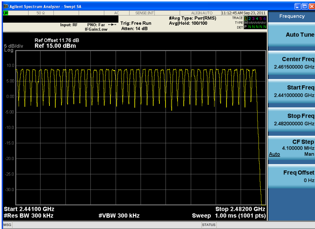
Plot 6-19. High End Spectrum Channel Hopping Plot (Bluetooth)
