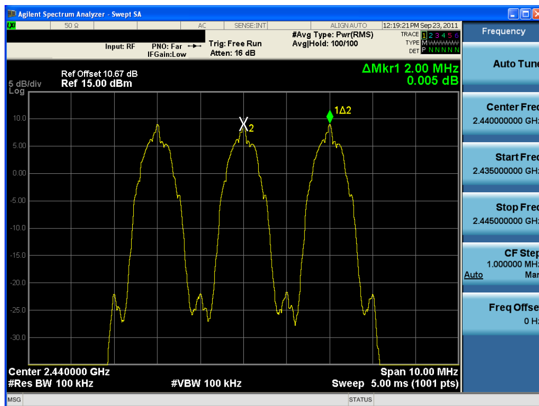
Plot 6-16. Channel Spacing Plot (Bluetooth LE Mode)
