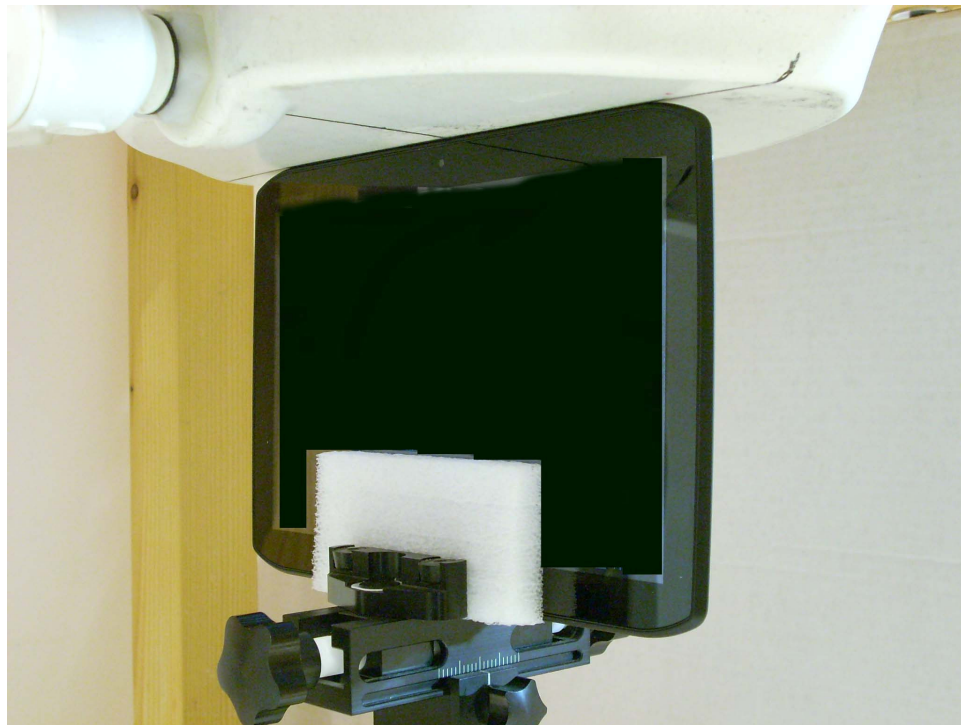
SAR Test Setup Photo 2 – Top at 0.0 cm
