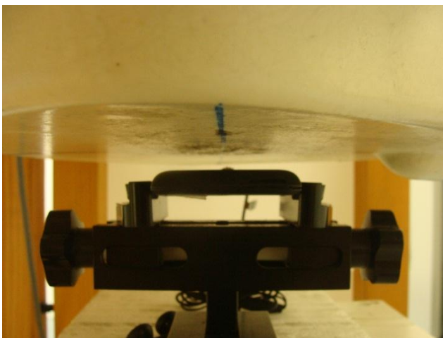
Back of the DUT with Phantom 1 cm Gap (DUT with Earphone)
