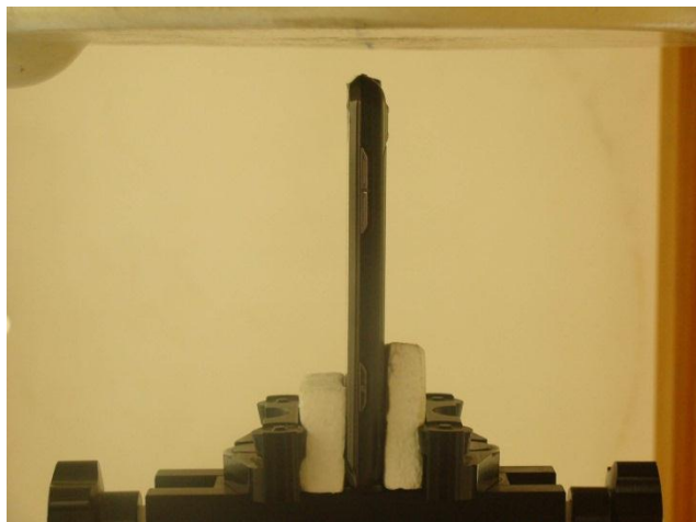
Top side of the DUT with Phantom 1 cm Gap (DUT without Earphone)
