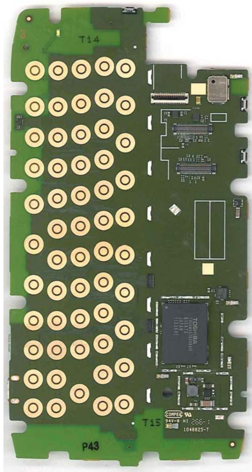
Main Board Top Without Shields
