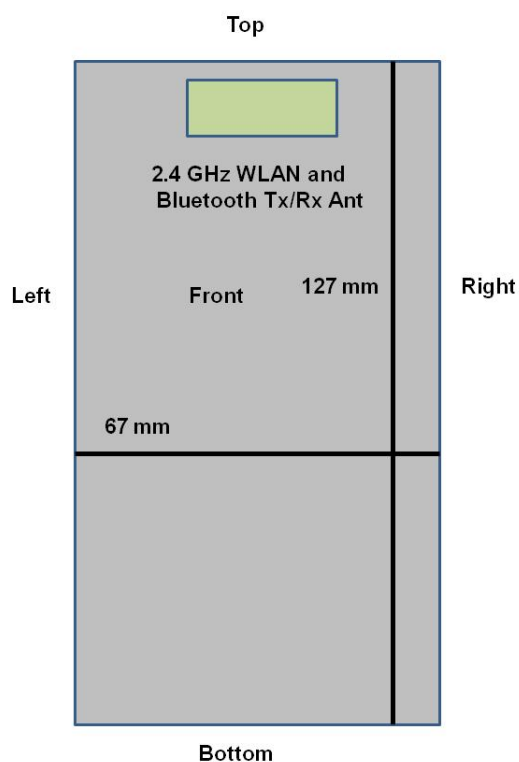
Figure 12-1 Identification of Sides for SAR Testing
