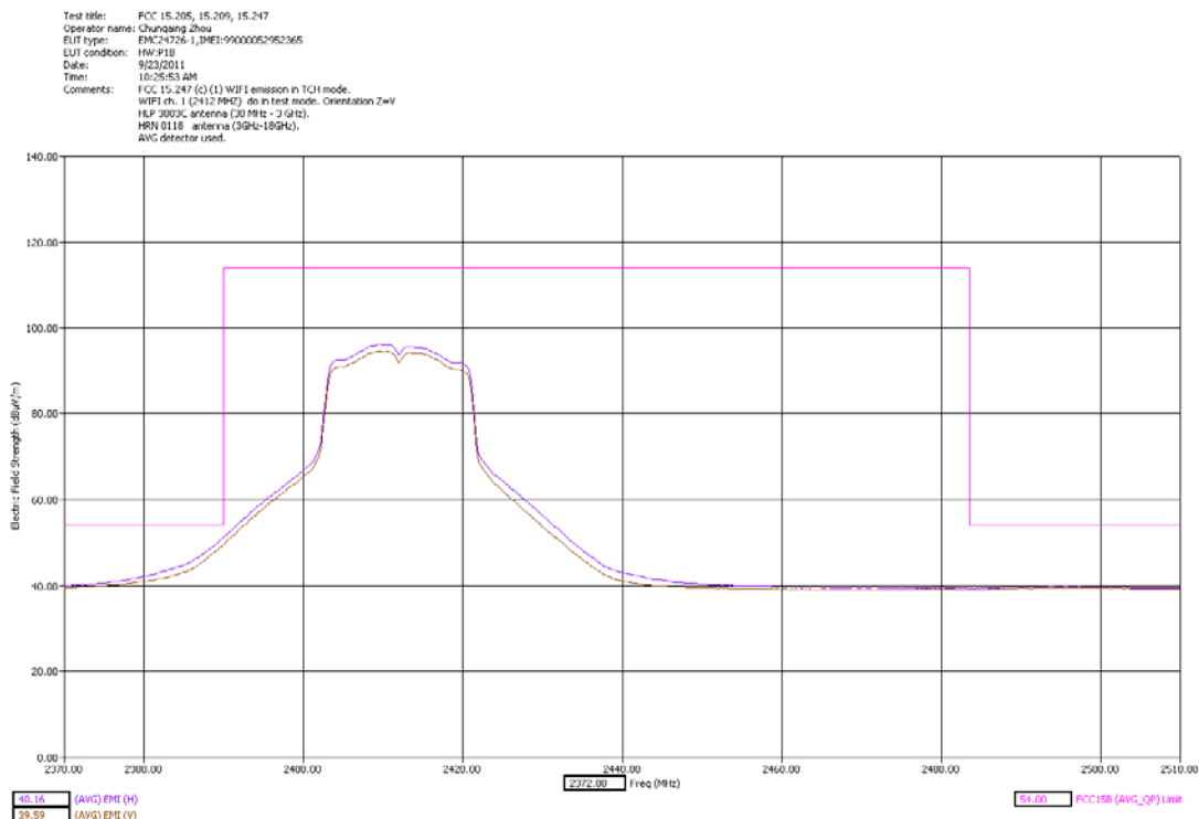
Low Channel Band Edge Z Orientation AVG Detector slider open
