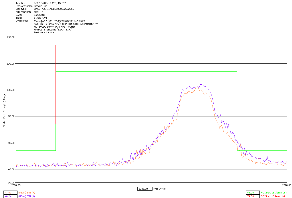
High Channel Band Edge Y Orientation Peak Detector slider close
