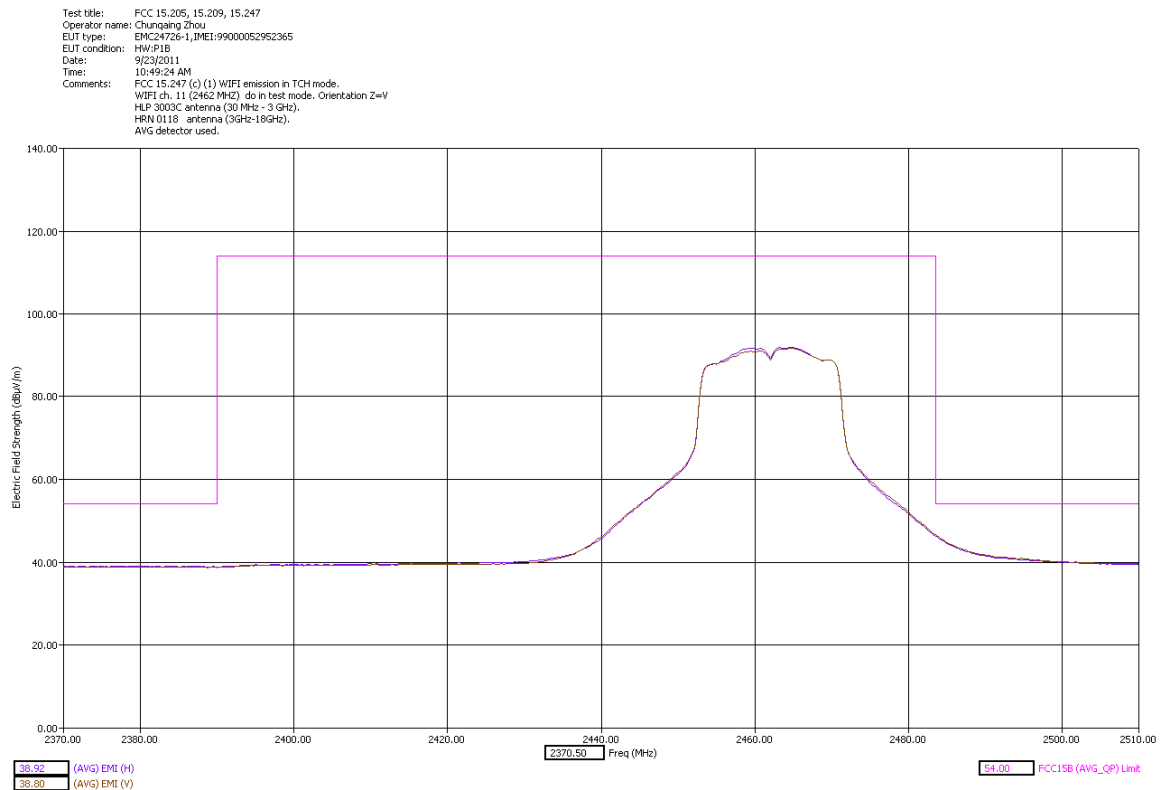
High Channel Band Edge Y Orientation AVG Detector slider close
