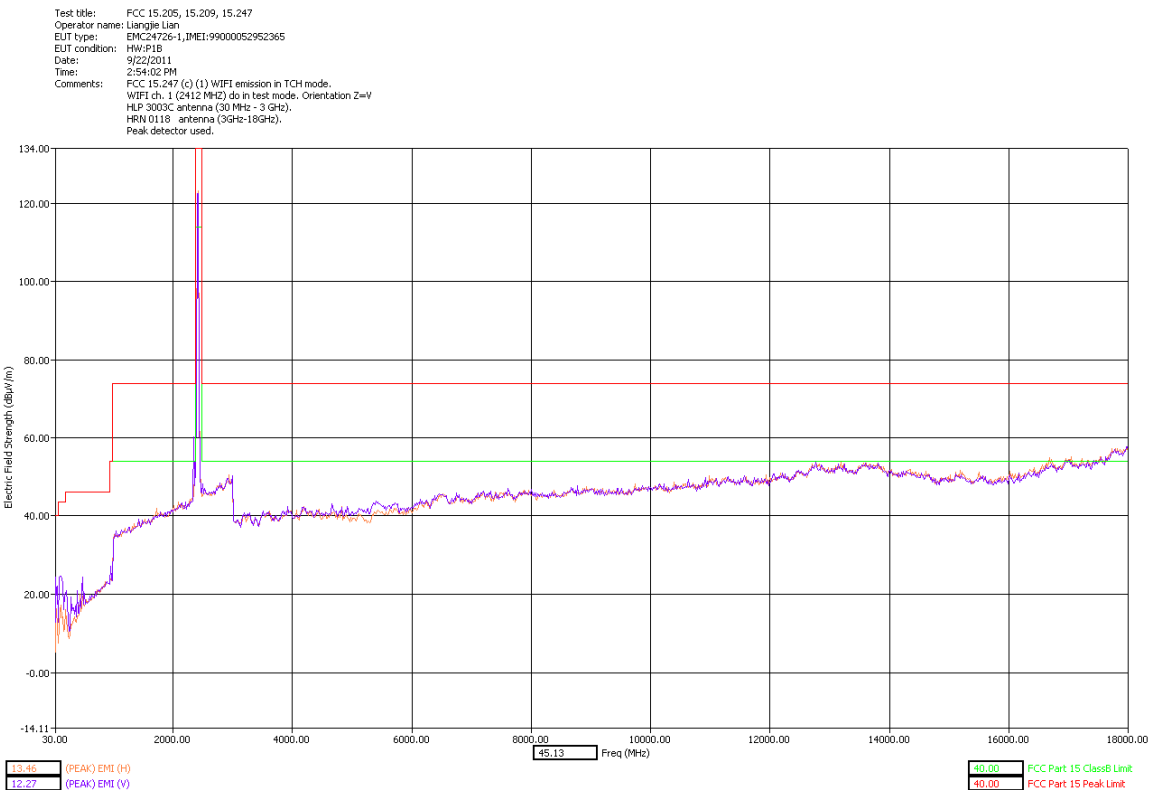
Low Channel Dual Polarization Y slider close
