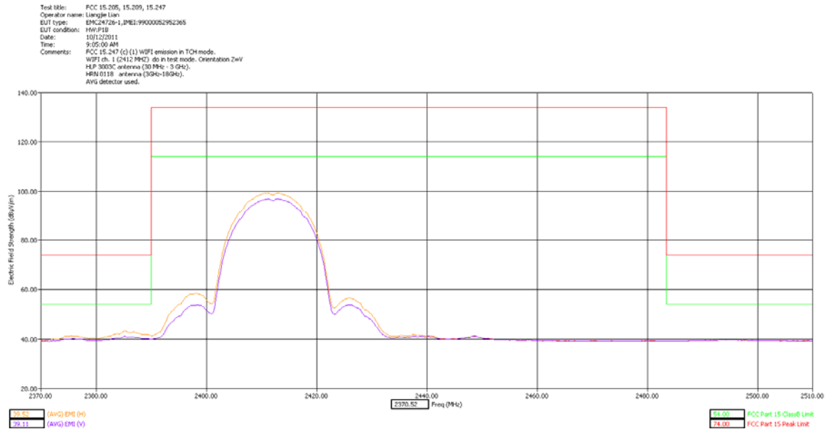
Low Channel Band Edge Y Orientation AVG Detector slider close
