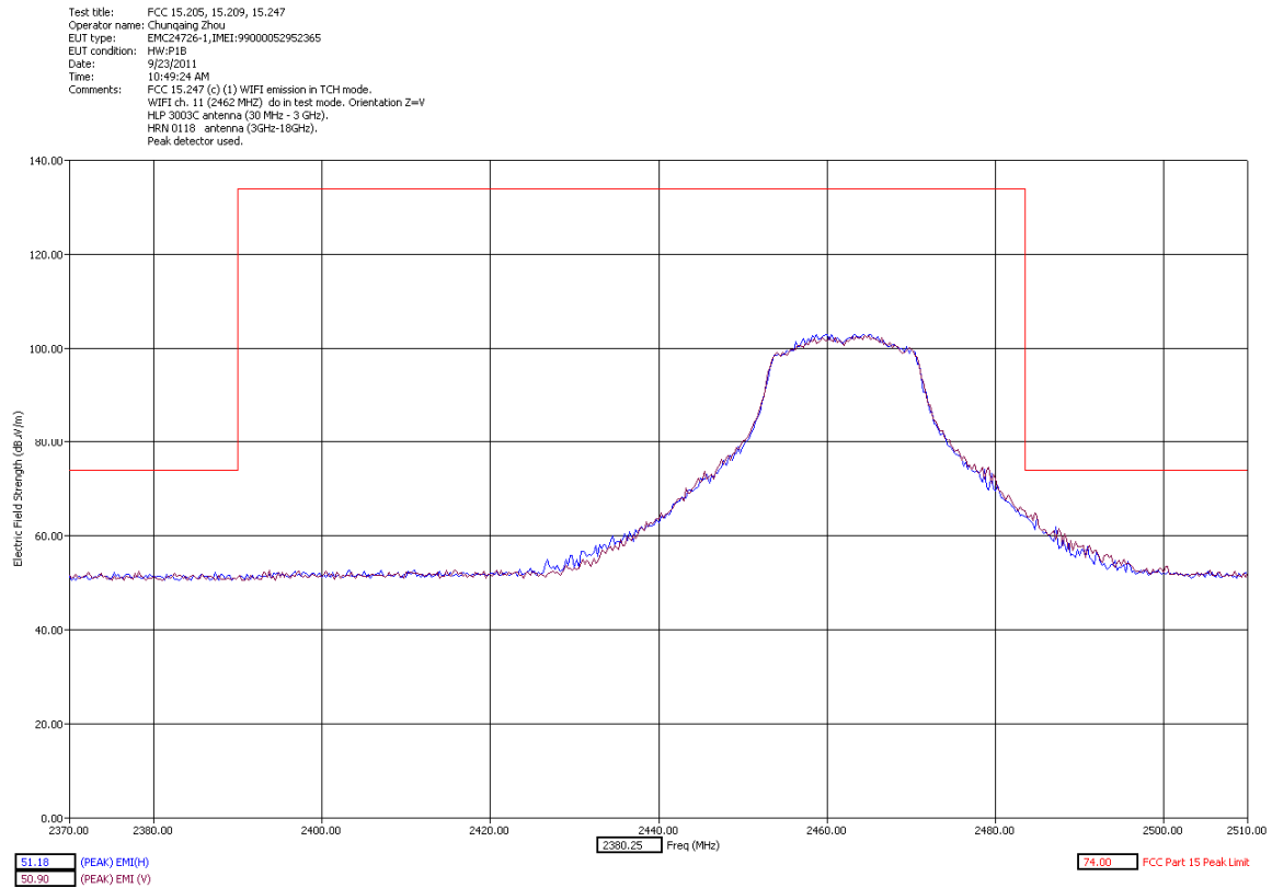
High Channel Band Edge Y Orientation Peak Detector slider close
