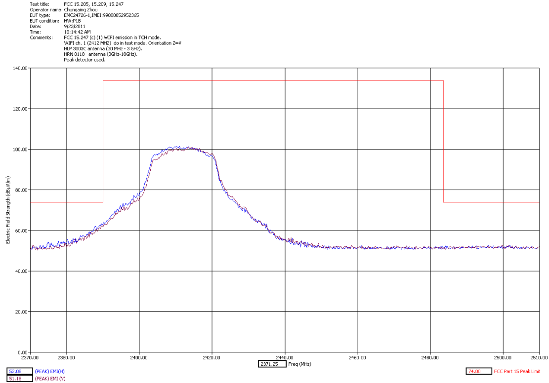
Low Channel Band Edge Y Orientation Peak Detector slider close
