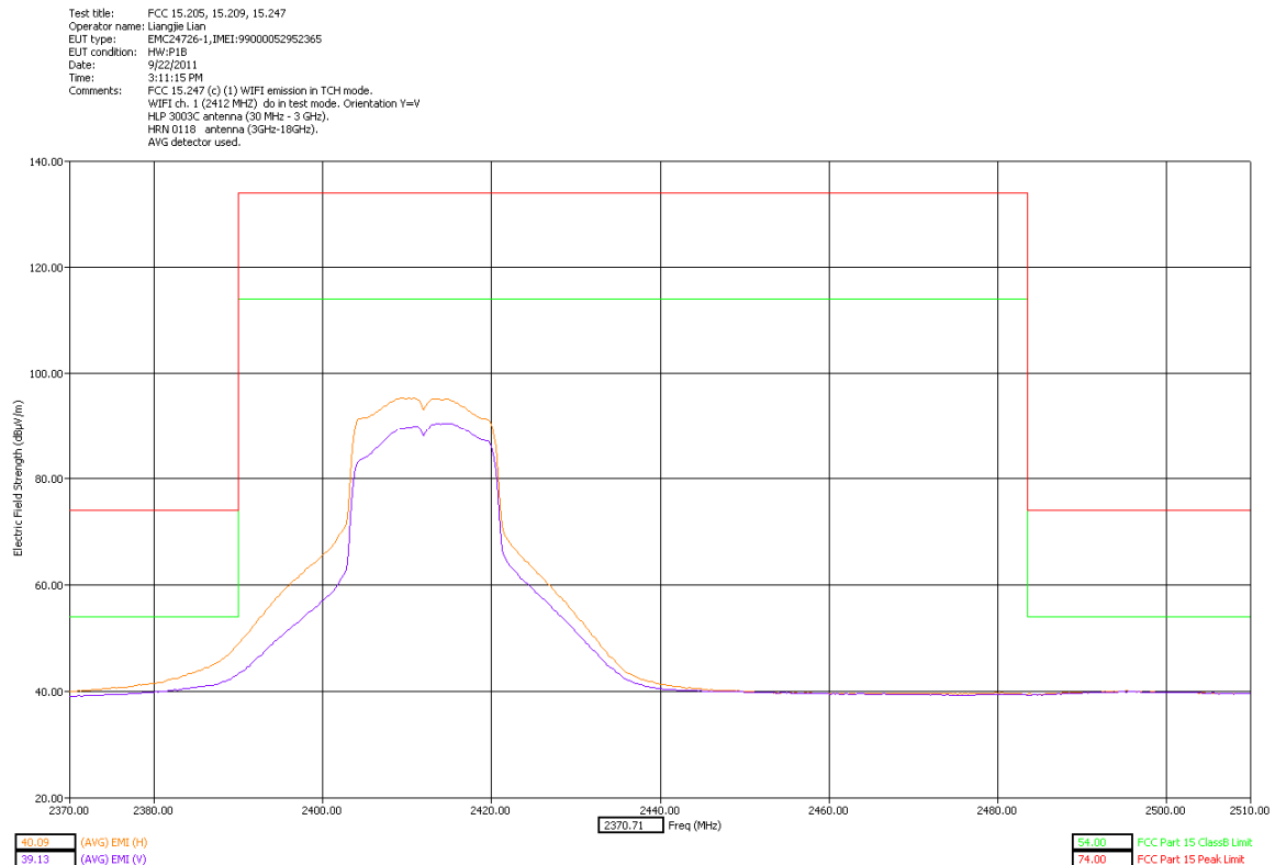
Low Channel Band Edge Y Orientation AVG Detector slider close
