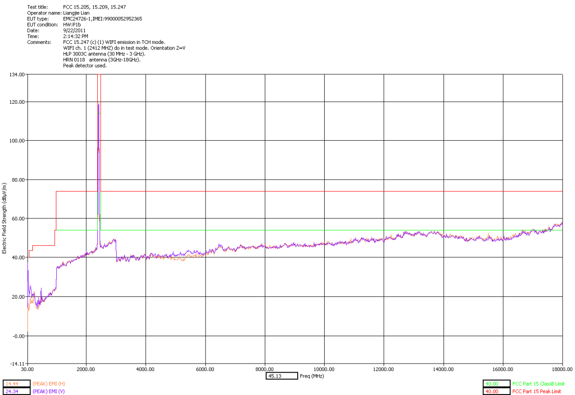
Low Channel Dual Polarization with the wireless charging battery cover
