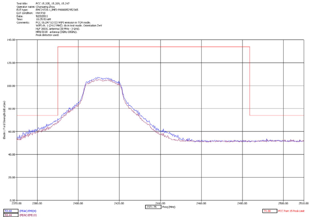
Low Channel Band Edge Z Orientation Peak Detector slider open
