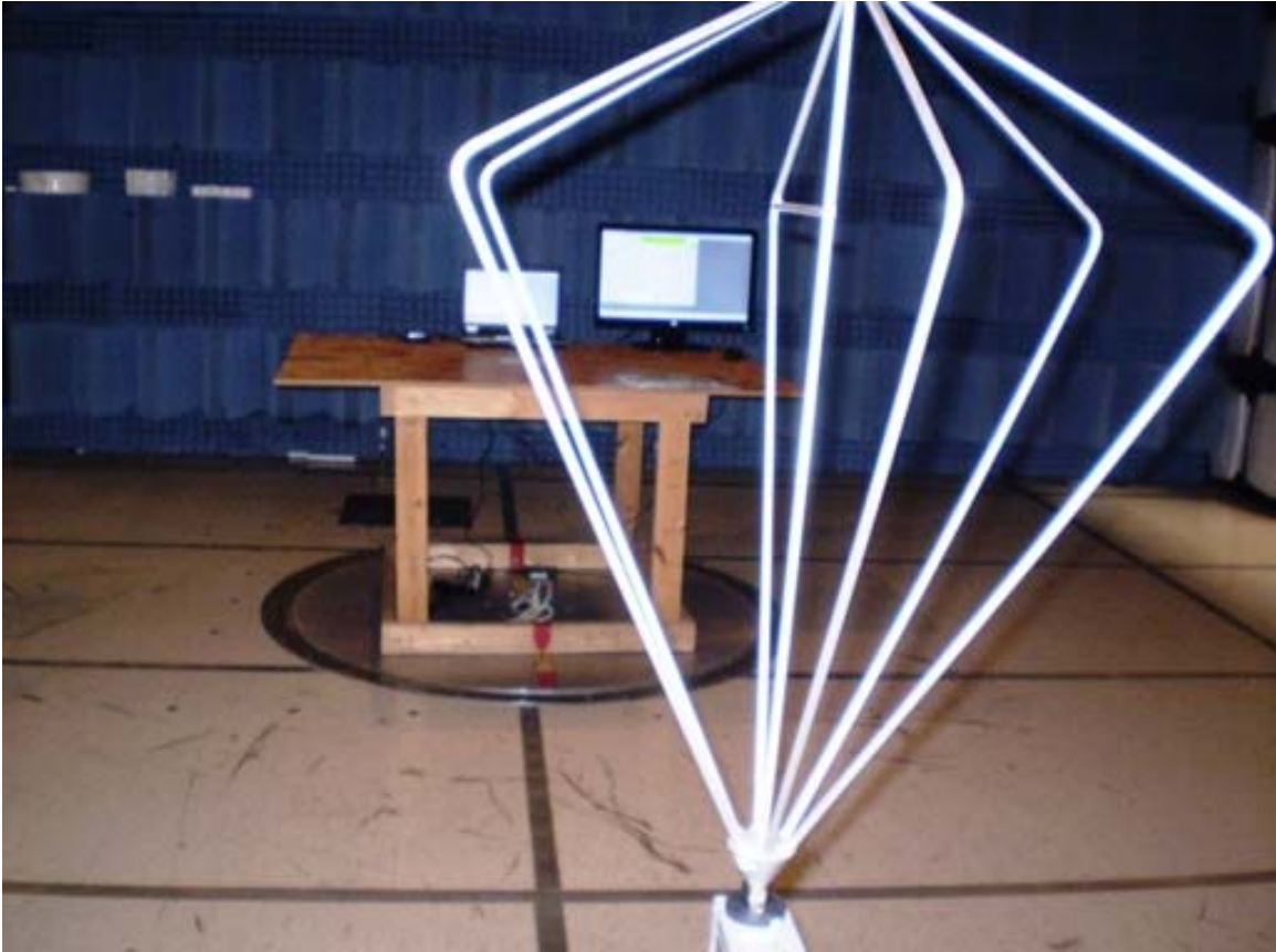
Radiated Emissions - Part 15 PC Peripheral with standard battery door
