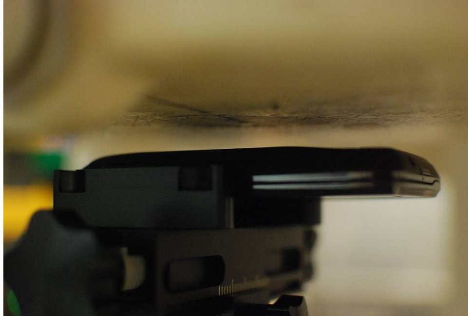
SAR Test Setup Photo 7 – Back at 1.0 cm with Inductive Cover
