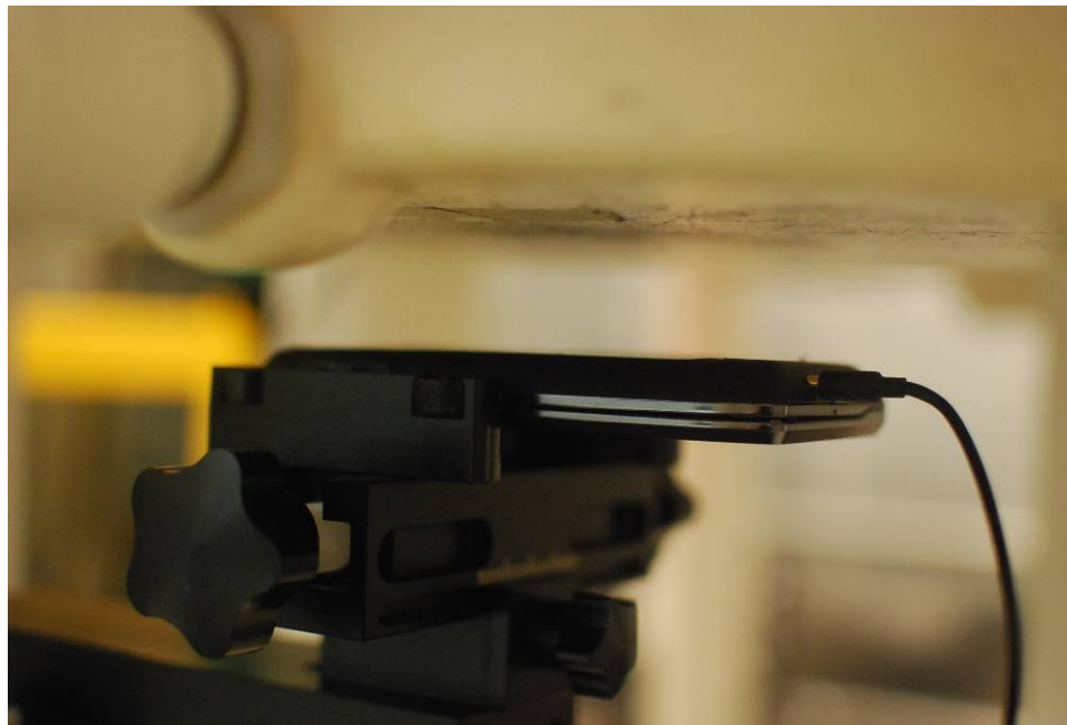
SAR Test Setup Photo 12 – Body Worn at 2.5 cm
