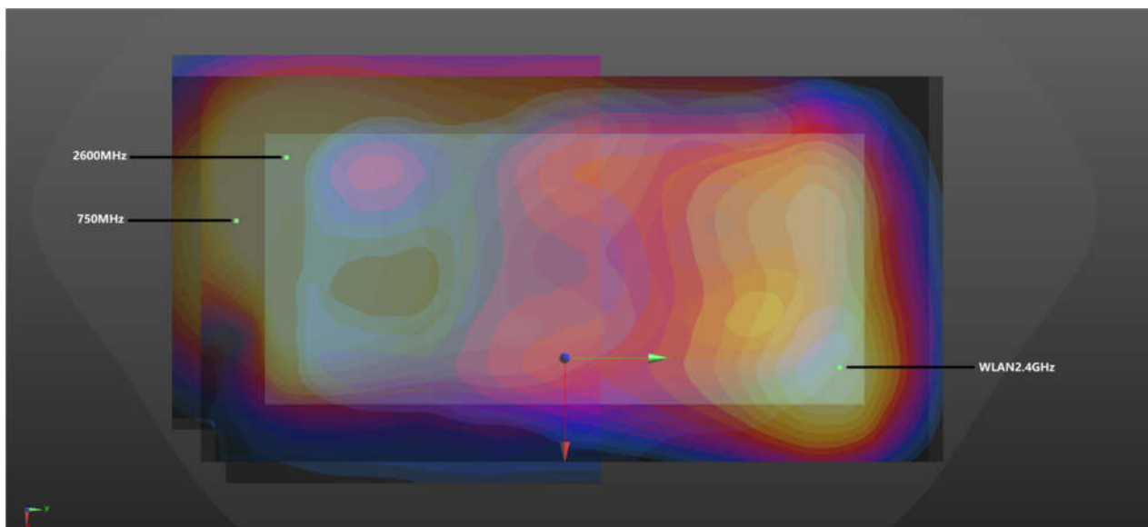
WWAN+WLAN2.4GHz_Front 5mm
