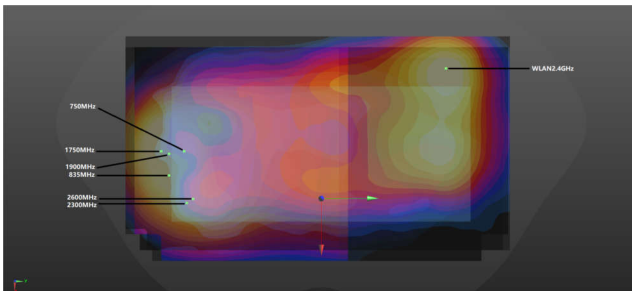
WWAN+WLAN2.4GHz_Back 5mm
