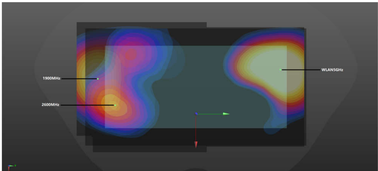
WWAN+WLAN5GHz_Back 22mm
