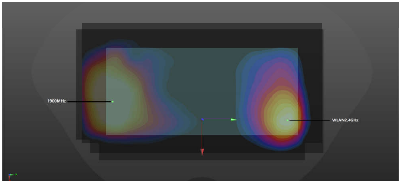
WWAN+WLAN2.4GHz_Front 0mm
