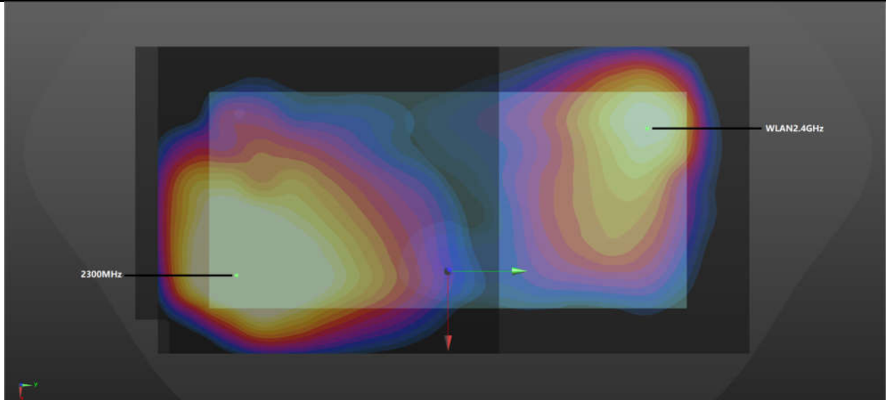
WWAN+WLAN2.4GHz_Back 0mm
