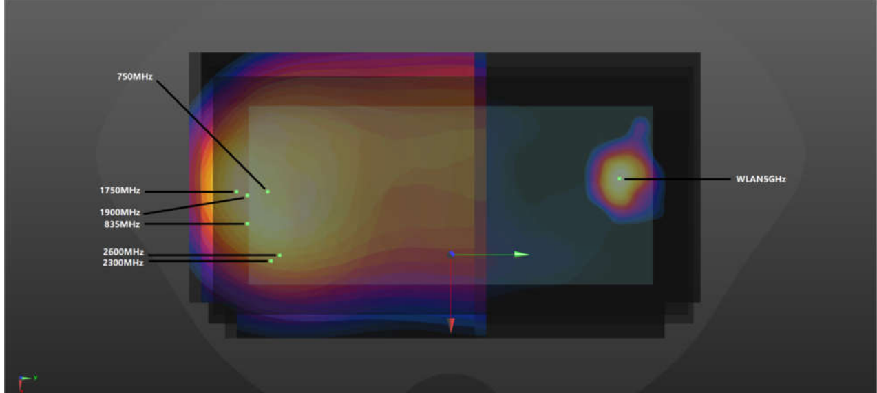
WWAN+WLAN5GHz_Back 5mm
