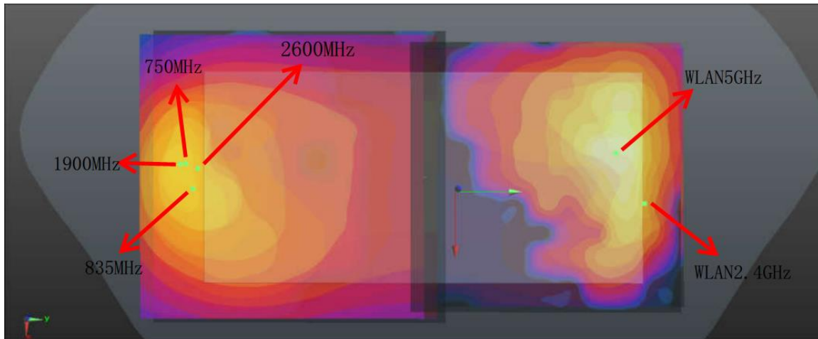
WWAN+WLAN2.4GHz/5GHz_5mm
