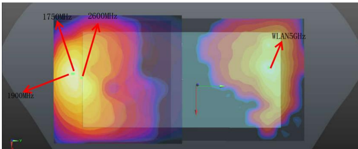
WWAN+WLAN5GHz_0mm
