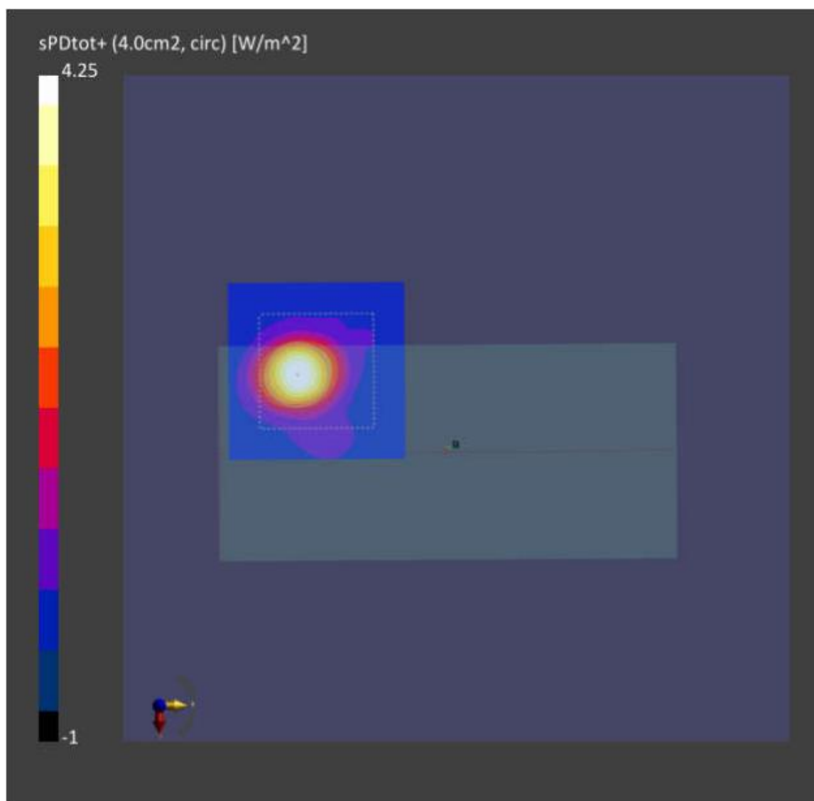
Figure 8-4: 4cm2-averaged power density distribution measured at input.power.limit of 4.25dBm on the back surface for n261 beam 41
