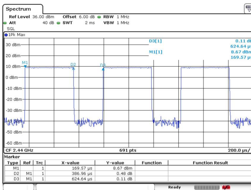
Bluetooth LE 1Mbps for ant4
