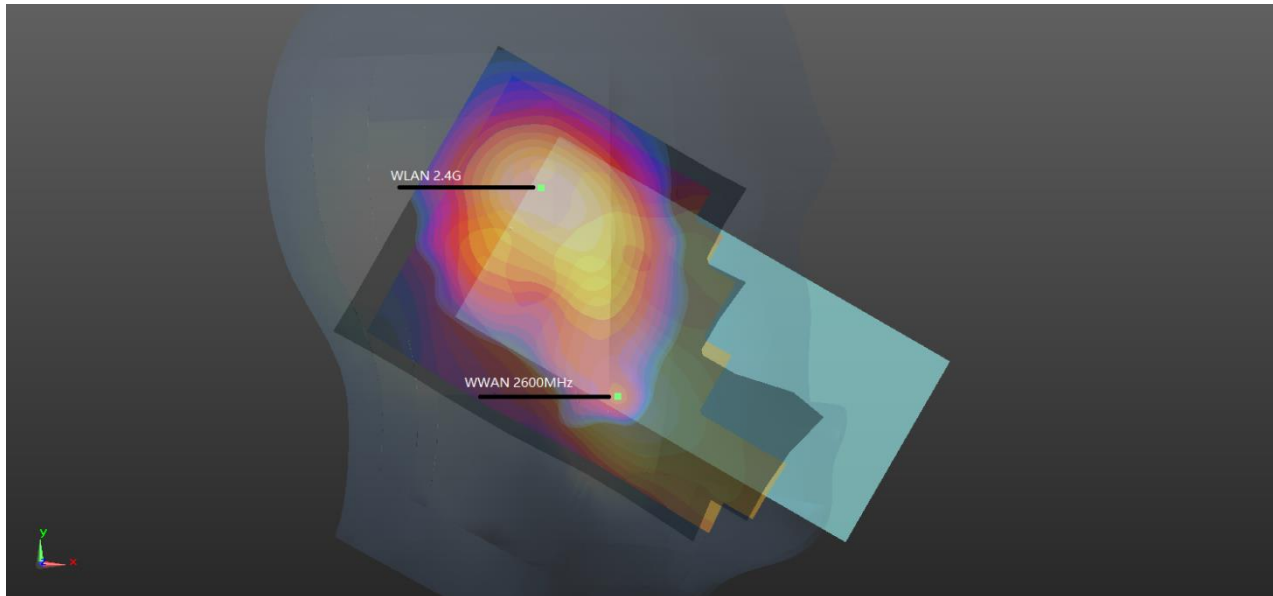
WWAN+ WLAN2.4GHz _ Head 0mm
