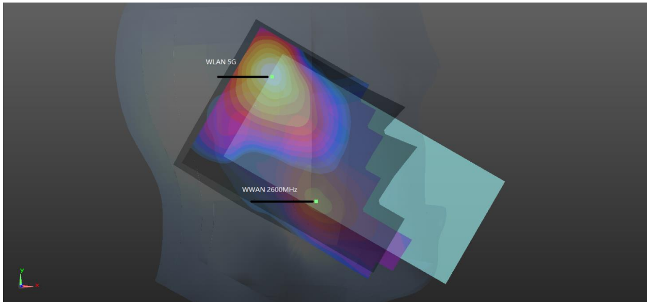
WWAN+ WLAN5GHz _ Head 0mm
