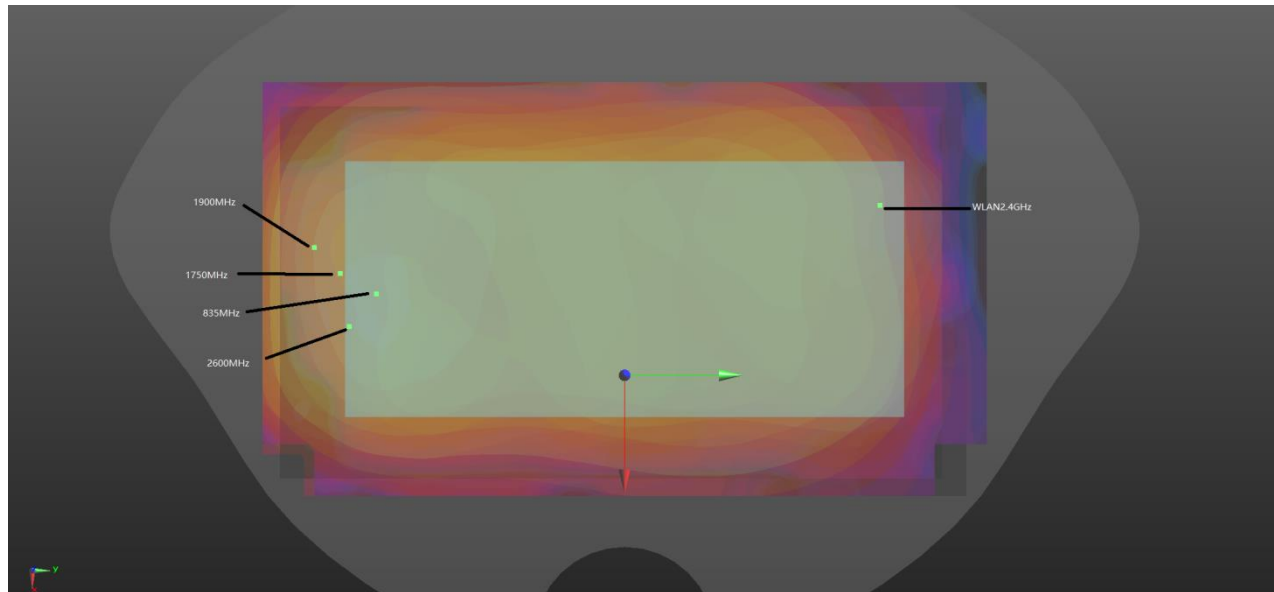
WWAN+WLAN2.4GHz_Back 5mm
