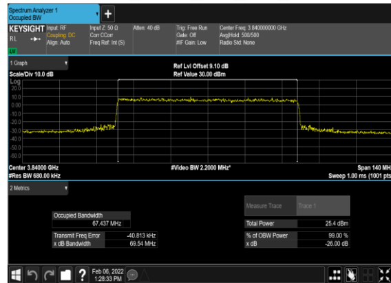
B41_N77(70M)_CP-OFDM_16QAM_Outer_Full_Mid_CH
