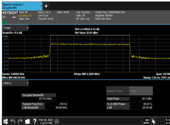
B41_N77(70M)_CP-OFDM_QPSK_Outer_Full_Mid_CH
