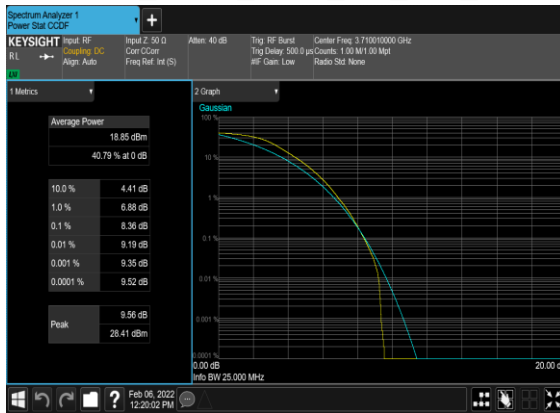
B41_N77(20M)_DFT-s-OFDM_QPSK_Outer_Full_Low_CH
