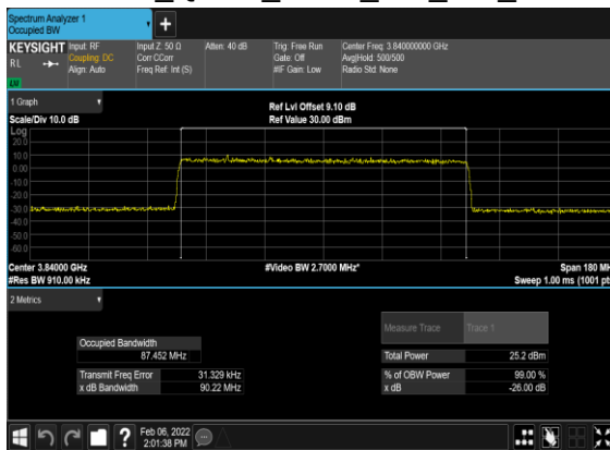
B41_N77(90M)_CP- OFDM_QPSK_Outer_Full_Mid_CH
