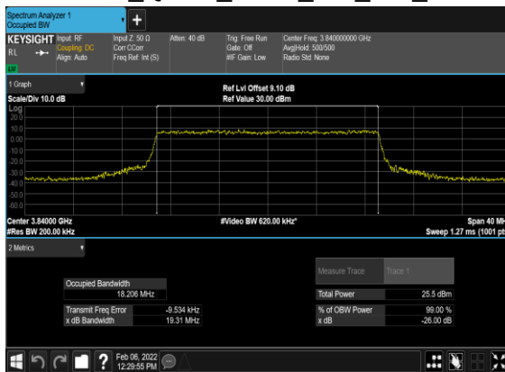
B41_N77(20M)_CP- OFDM_QPSK_Outer_Full_Mid_CH
