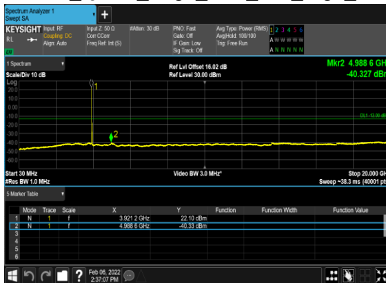
B41_N77(60M)_DFT-s- OFDM_QPSK_Edge_1RB_Left_High_CH
