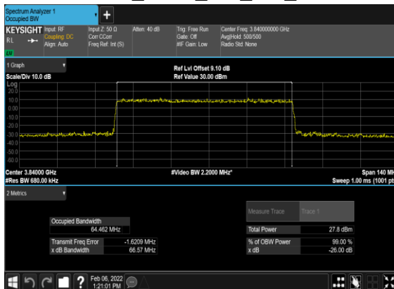
B41_N77(70M)_DFT-s-OFDM_PI-2-BPSK_Outer_Full_Mid_CH
