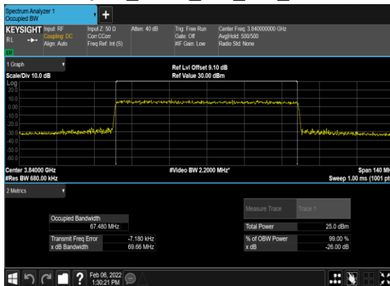
B41_N77(70M)_CP-OFDM_64QAM_Outer_Full_Mid_CH
