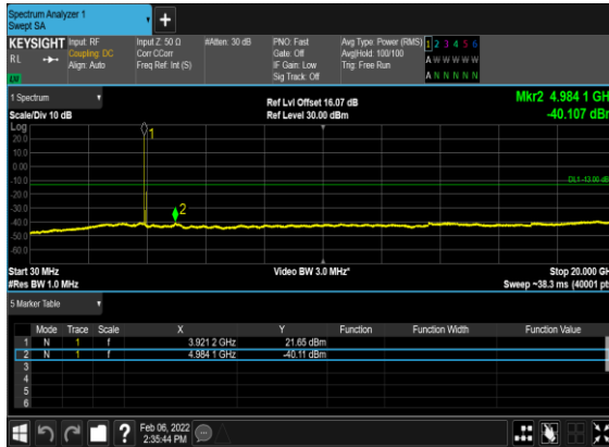
B41_N77(60M)_DFT-s- OFDM_BPSK_Edge_1RB_Left_High_CH
