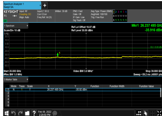
B41_N77(60M)_DFT-s- OFDM_BPSK_Edge_1RB_Left_Low_CH
