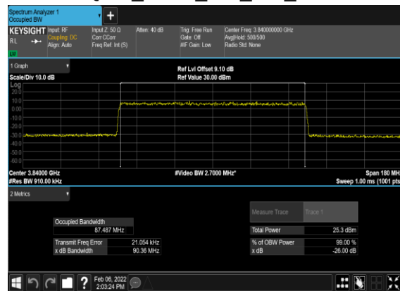
B41_N77(90M)_CP-OFDM_16 QAM_Outer_Full_Mid_CH
