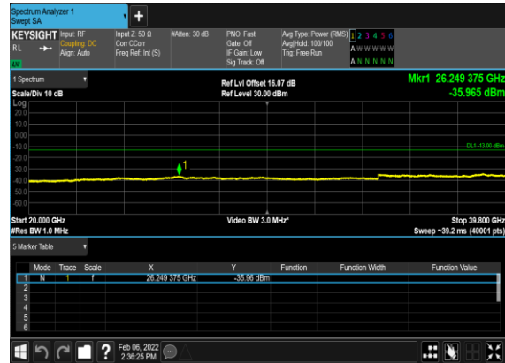
B41_N77(60M)_DFT-s- OFDM_BPSK_Edge_1RB_Left_High_CH
