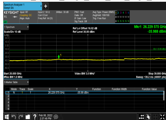
B41_N77(60M)_DFT-s- OFDM_QPSK_Edge_1RB_Left_High_CH
