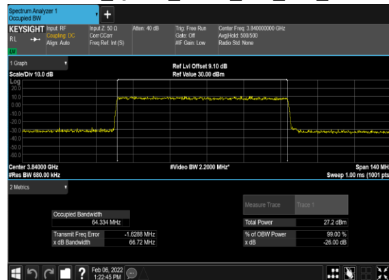
B41_N77(70M)_DFT-s-OFDM_QPSK_Outer_Full_Mid_CH
