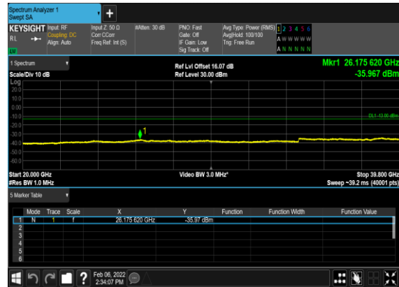
B41_N77(60M)_DFT-s- OFDM_QPSK_Edge_1RB_Left_Mid_CH
