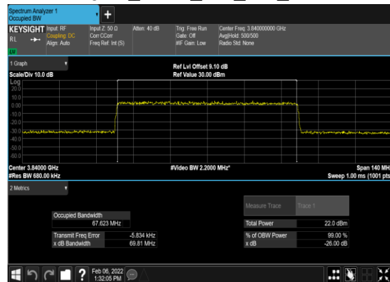
B41_N77(70M)_CP-OFDM_256QAM_Outer_Full_Mid_CH
