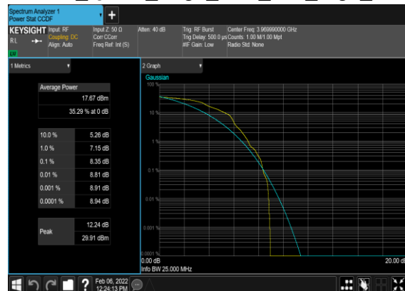
B41_N77(20M)_DFT-s-OFDM_QPSK_Edge_1RB_Left_High_CH
