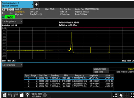
B41_N77(60M)_DFT-s- OFDM_QPSK_Edge_1RB_Left_Low_CH
