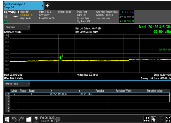
B41_N77(100M)_DFT-s-OFDM_QPSK_Edge_1RB_Left_Mid_CH
