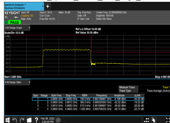
B41_N77(60M)_DFT-s- OFDM_QPSK_Outer_Full_High_CH
