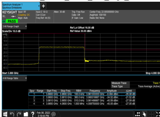
B41_N77(60M)_DFT-s- OFDM_BPSK_Outer_Full_High_CH
