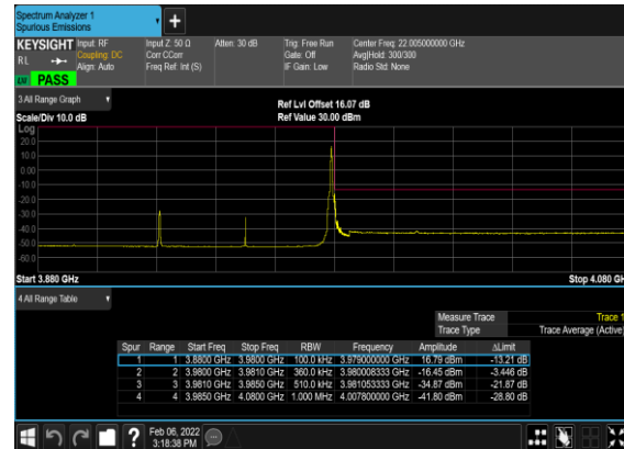
B41_N77(60M)_DFT-s- OFDM_QPSK_Edge_1RB_Right_High_CH
