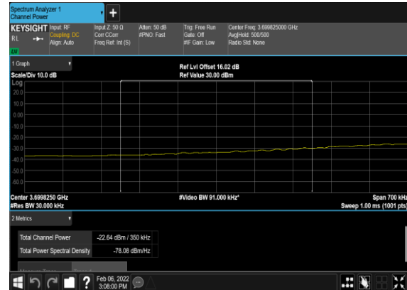
B41_N77(60M)_DFT-s- OFDM_QPSK_Edge_1RB_Left_Low_CH_CHP_PA SS
