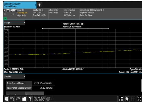
B41_N77(60M)_DFT-s- OFDM_BPSK_Edge_1RB_Left_Low_CH_CHP_PA SS
