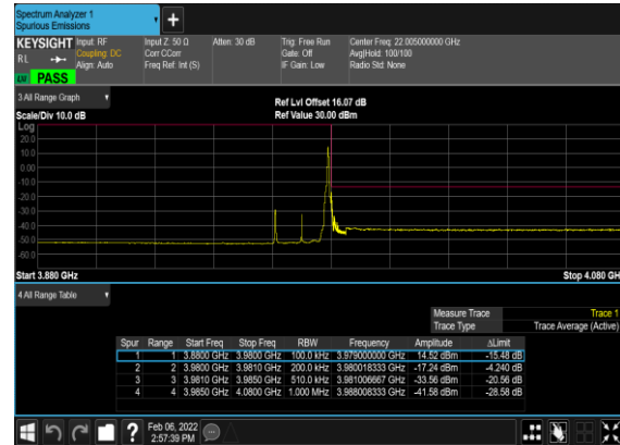
B41_N77(20M)_DFT-s- OFDM_QPSK_Edge_1RB_Right_High_CH
