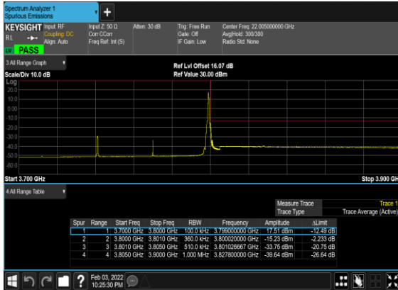
N78(60M)_DFT-s-OFDM_QPSK_Edge_1RB_Right_High_CH
