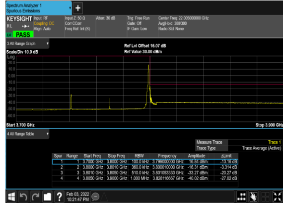
N78(60M)_DFT-s-OFDM_BPSK_Edge_1RB_Right_High_CH
