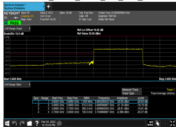
N78(60M)_DFT-s- OFDM_BPSK_Outer_Full_Low_CH
