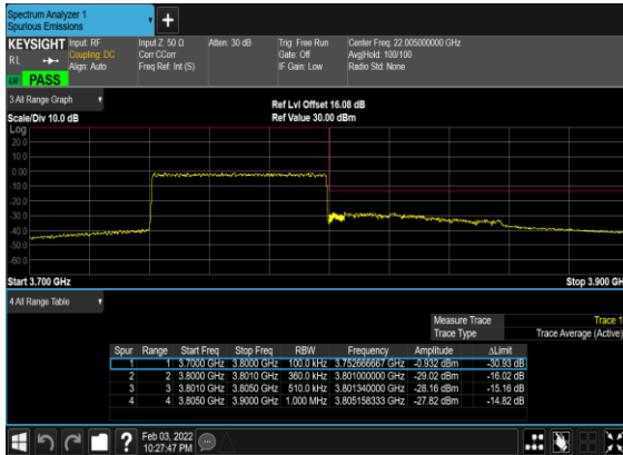
N78(60M)_DFT-s-OFDM_QPSK_Outer_Full_High_CH
