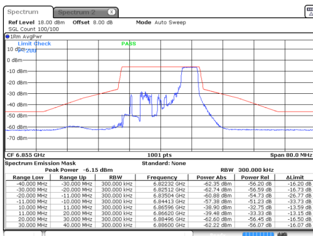
Plot on Channel 6855MHz 52RU40
