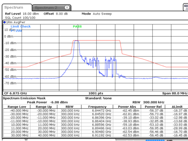
Plot on Channel 6875MHz 26RU0
