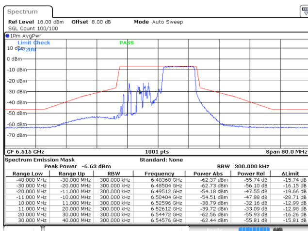
Plot on Channel 6515MHz 106RU54
