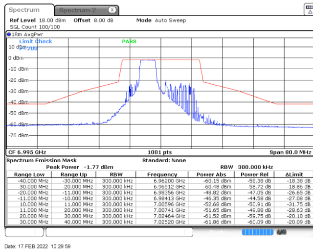
Plot on Channel 6995MHz 52RU38
