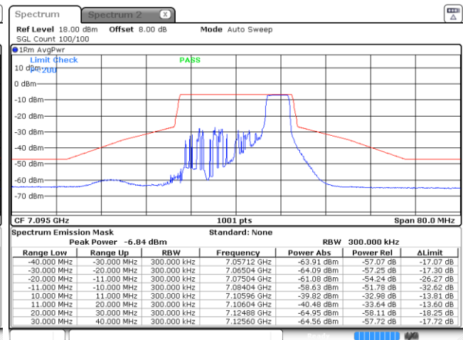
Plot on Channel 7095MHz 52RU40
