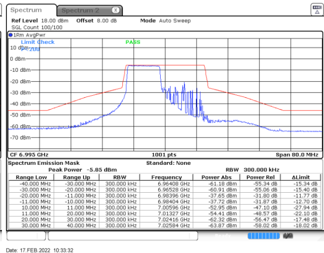
Plot on Channel 6995MHz 106RU53
