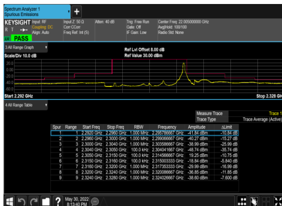
N30(10M)_DFT-s-OFDM_BPSK_Edge_1RB_Right_Low_CH N30(10M)_DFT-s-OFDM_QPSK_Edge_1RB_Right_Low_CH
