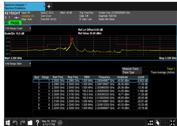
N30(10M)_DFT-s-OFDM_QPSK_Edge_1RB_Left_Low_CH
