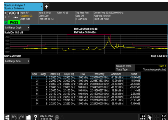
N30(10M)_DFT-s-OFDM_BPSK_Edge_1RB_Right_Low_CH N30(10M)_DFT-s-OFDM_QPSK_Edge_1RB_Right_Low_CH
