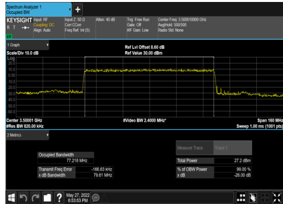
N77(80M)_DFT-s- OFDM_QPSK_Outer_Full_Mid_CH
