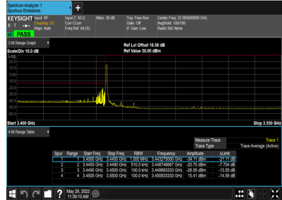
N77(10M)_DFT-s- OFDM_QPSK_Edge_1RB_Left_Low_CH
