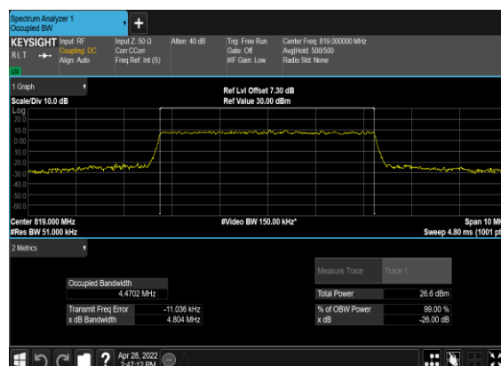
N26(5M)_CP-OFDM_16 QAM_Outer_Full_Mid_CH
